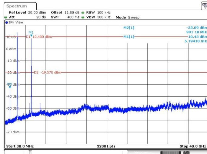
Conducted Emission Plots of chain 1
