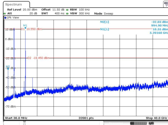
Conducted Emission Plots of chain 0
