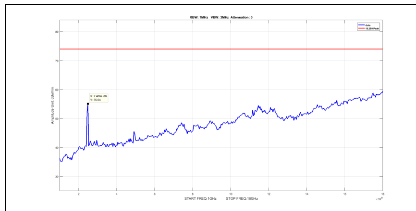
Plot 63. Radiated Emissions, pk, n mode, 2452MHz, 1G-18G
