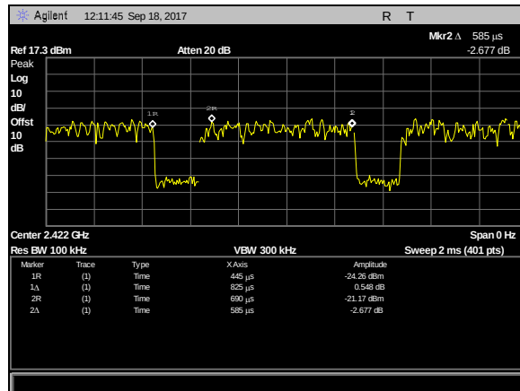
Plot 96. n mode, 40MHzBW, Duty Cycle
