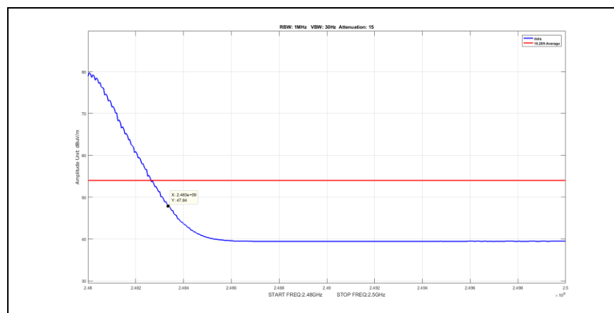
Plot 79. Radiated Emissions, BT band edge DH5 high 7 avg
