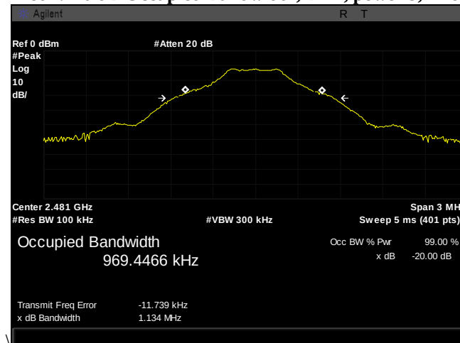
Plot 3. 20 dB Occupied Bandwidth, DH1, power 9, High
