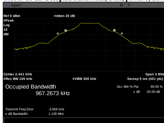
Plot 2. 20 dB Occupied Bandwidth, DH1, power 9, Mid
