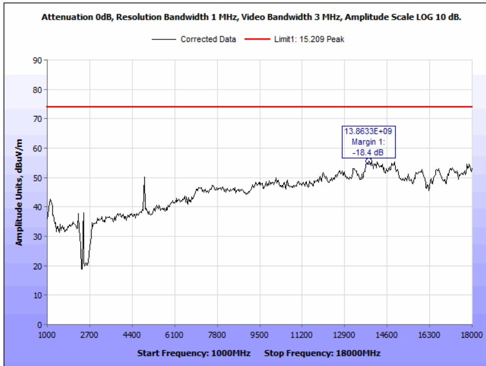
Figure 30: PK_Radiated Emissions_802.11g_2437Mz_1-18GHz.
