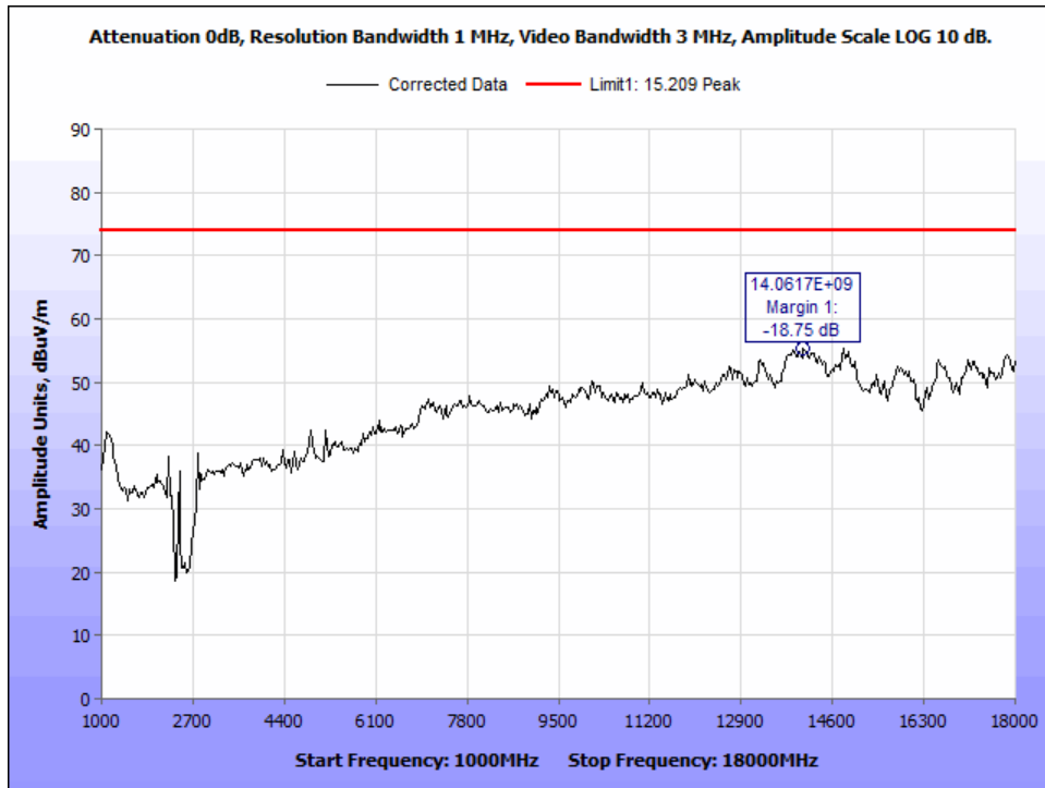
Figure 36: PK_Radiated Emissions_802.11n40_2437Mz_1-18GHz.
