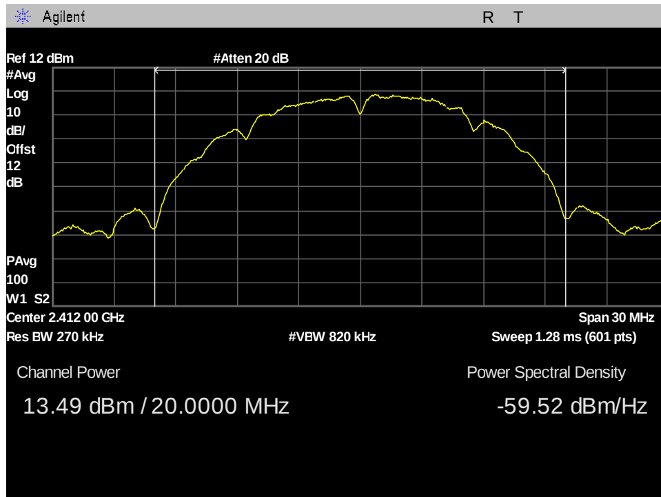
Figure 63: OP_802.11b_2412MHz
