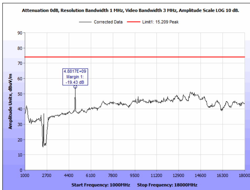
Figure 27: PK_Radiated Emissions_802.11b_2437Mz_1-18GHz.
