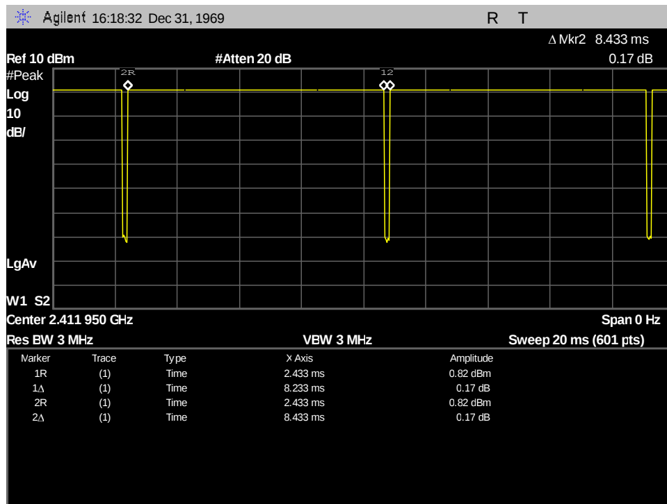
Figure 62: 802.11b DC
