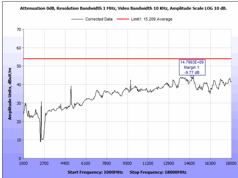
Figure 18: AVG_Radiated Emissions_802.11g_2437Mz_1-18GHz.
