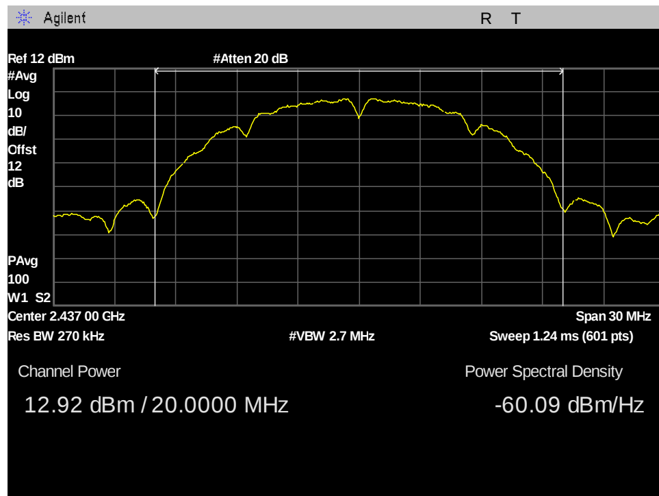
Figure 64: OP_802.11b_2437MHz
