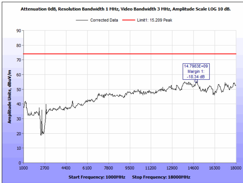
Figure 37: PK_Radiated Emissions_802.11n40_2452Mz_1-18GHz.
