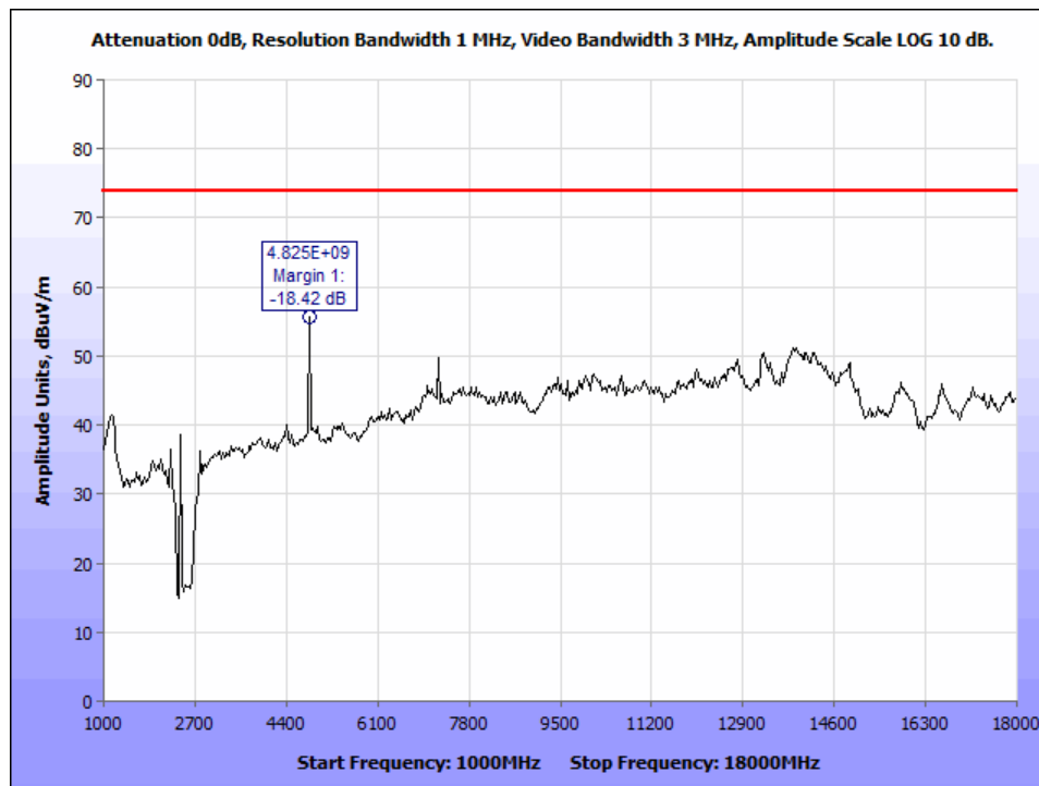
Figure 26: PK_Radiated Emissions_802.11b_2412Mz_1-18GHz.
