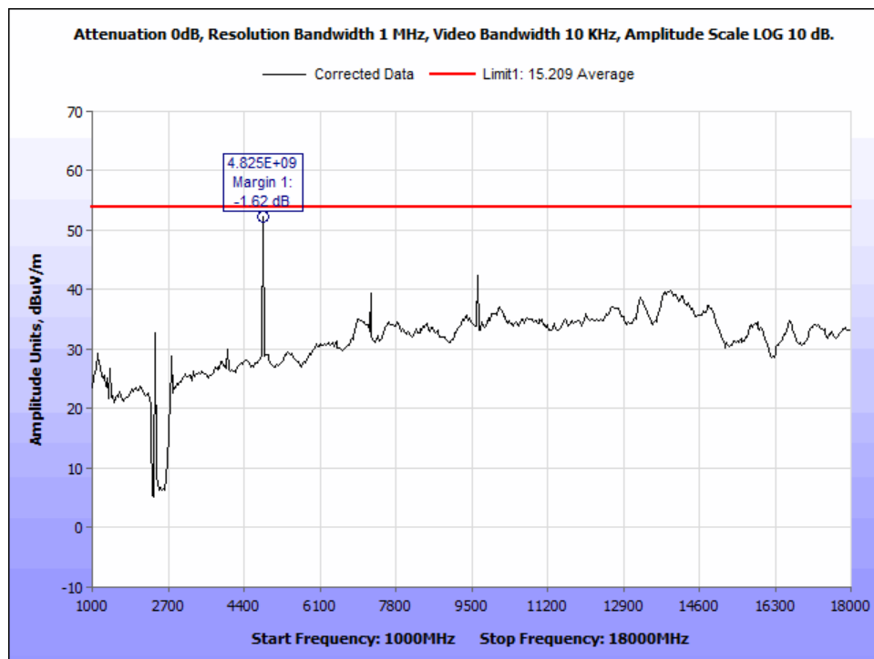
Figure 11: AVG_Radiated Emissions_802.11b_2412Mz_1-18GHz.
