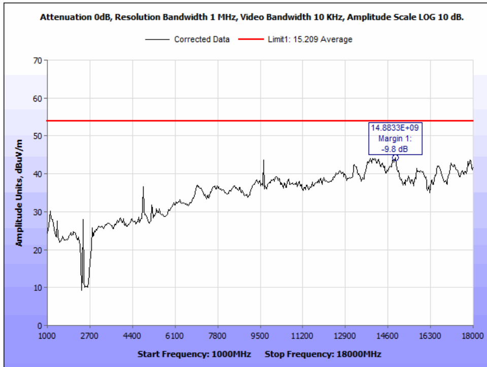
Figure 20: AVG_Radiated Emissions_802.11n20_2412Mz_1-18GHz.
