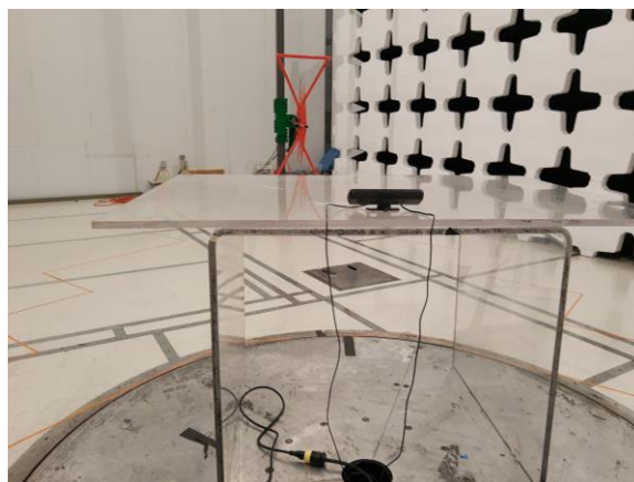
Figure 41: REE Test Setup - 30-1000MHz
