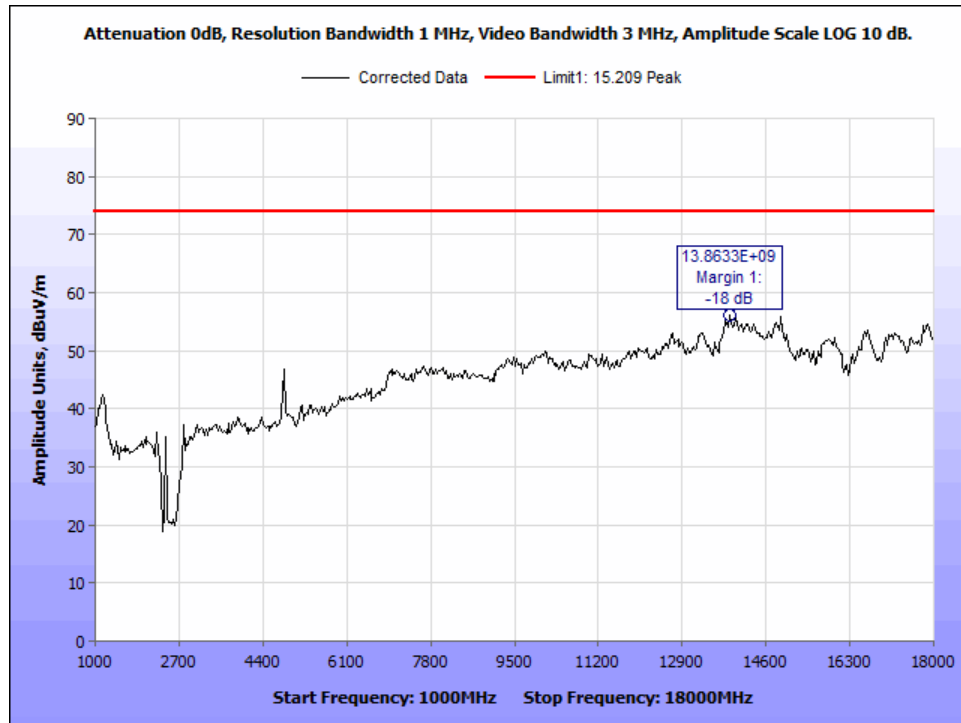
Figure 32: PK_Radiated Emissions_802.11n20_2412Mz_1-18GHz.
