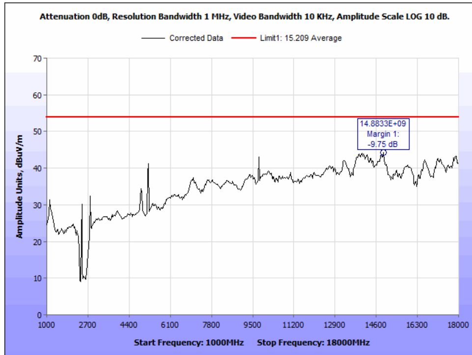
Figure 24: AVG_Radiated Emissions_802.11n40_2437Mz_1-18GHz.
