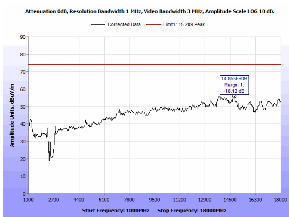
Figure 35: PK_Radiated Emissions_802.11n40_2422Mz_1-18GHz.
