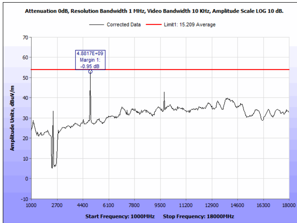
Figure 13: AVG_Radiated Emissions_802.11b_2437Mz_1-18GHz.
