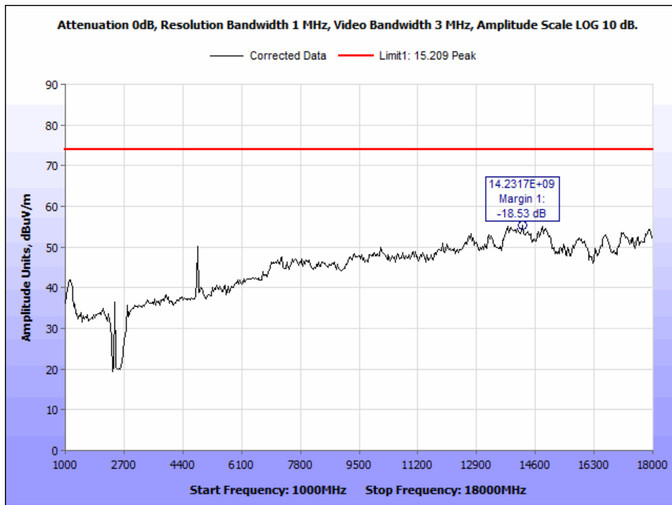
Figure 29: PK_Radiated Emissions_802.11g_2412Mz_1-18GHz.
