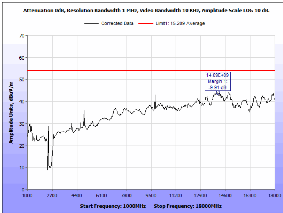
Figure 21: AVG_Radiated Emissions_802.11n20_2437Mz_1-18GHz.
