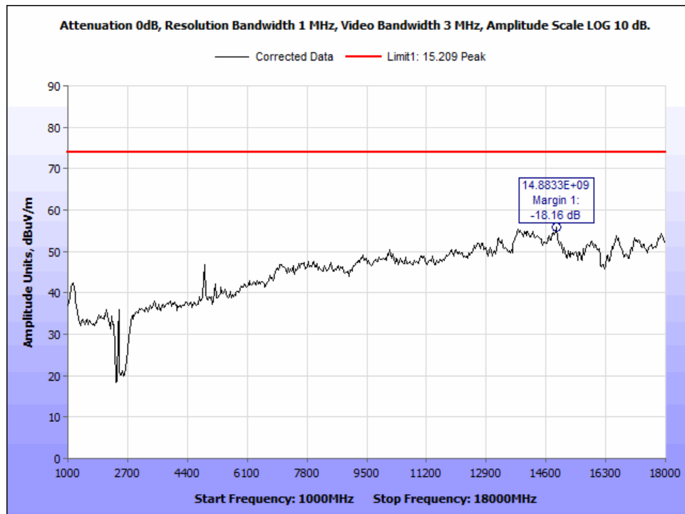
Figure 33: PK_Radiated Emissions_802.11n20_2437Mz_1-18GHz.
