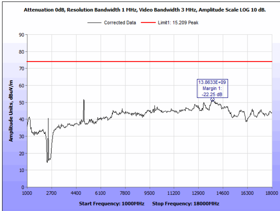
Figure 28: PK_Radiated Emissions_802.11b_2462Mz_1-18GHz.
