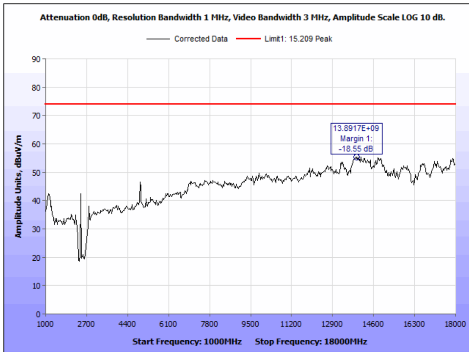
Figure 31: PK_Radiated Emissions_802.11g_2462Mz_1-18GHz.
