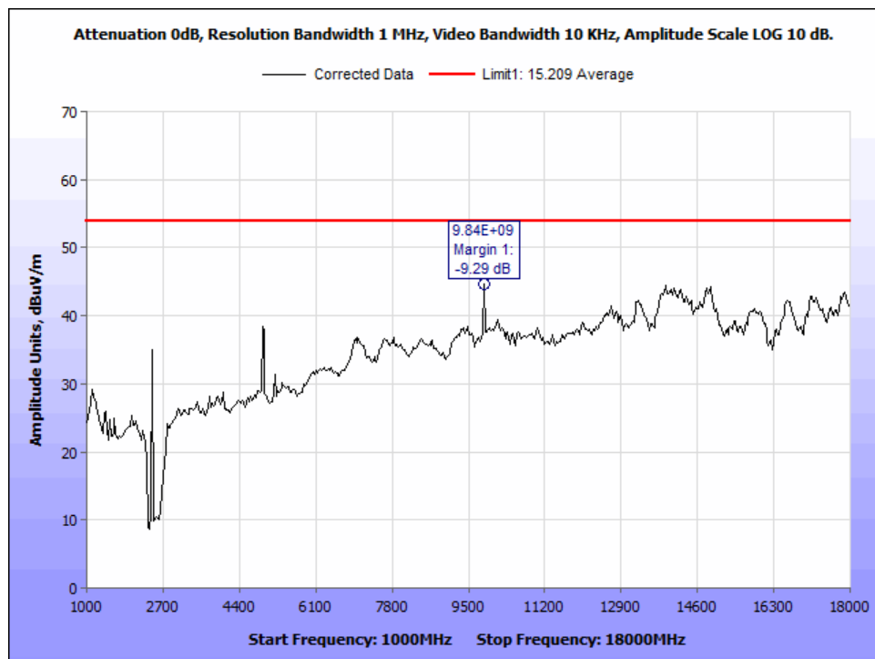
Figure 19: AVG_Radiated Emissions_802.11g_2462Mz_1-18GHz.
