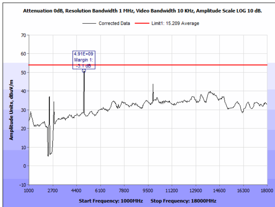
Figure 15: AVG_Radiated Emissions_802.11b_2462Mz_1-18GHz.
