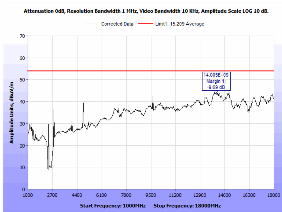
Figure 17: AVG_Radiated Emissions_802.11g_2412Mz_1-18GHz.
