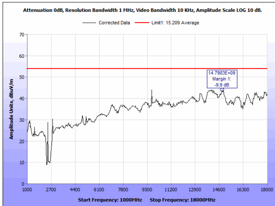
Figure 25: AVG_Radiated Emissions_802.11n40_2452Mz_1-18GHz.
