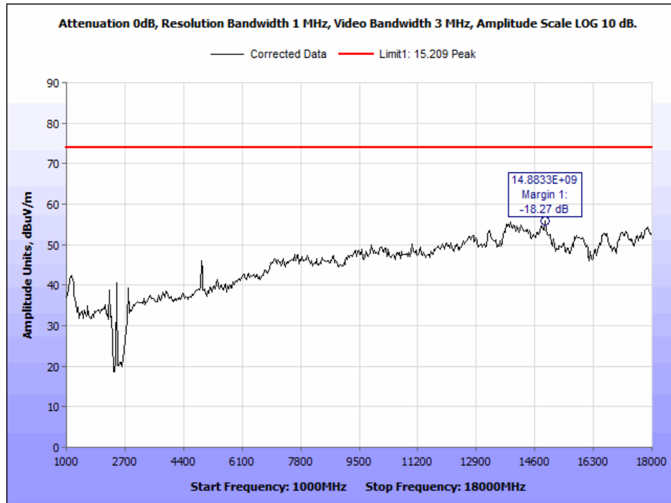
Figure 34: PK_Radiated Emissions_802.11n20_2462Mz_1-18GHz.
