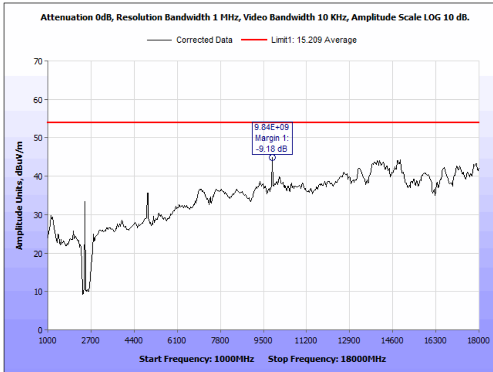
Figure 22: AVG_Radiated Emissions_802.11n20_2462Mz_1-18GHz.
