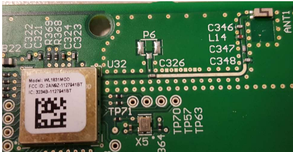
Radio module with matching network and antenna
