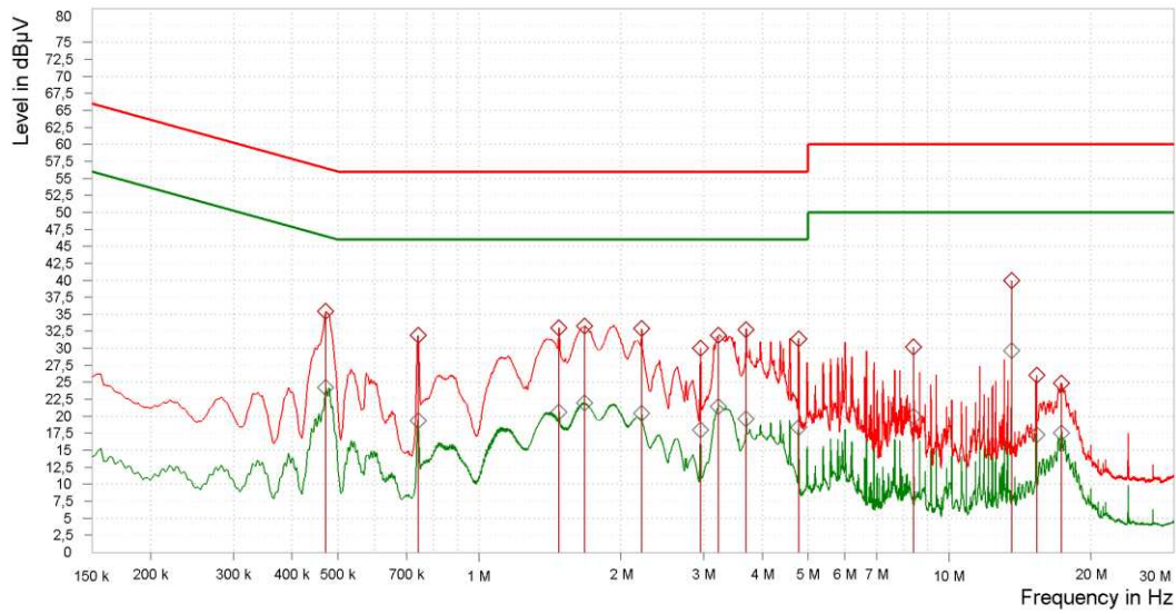
Plot No. 19: Conducted emissions, set-up 3, Op. 1, N
