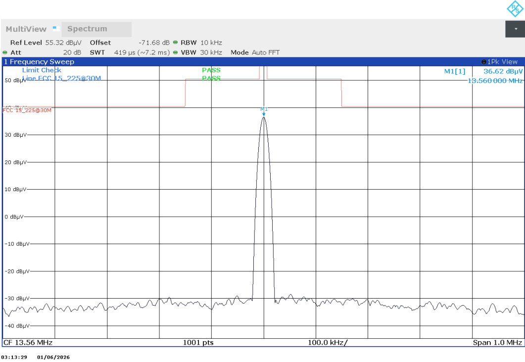
Plot no. 1: Transmitter Spectrum Mask (TSM), Set-up 1, Op. 1
