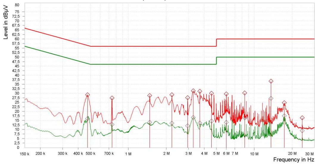
Plot No. 18: Conducted emissions, set-up 3, Op. 1, L1
