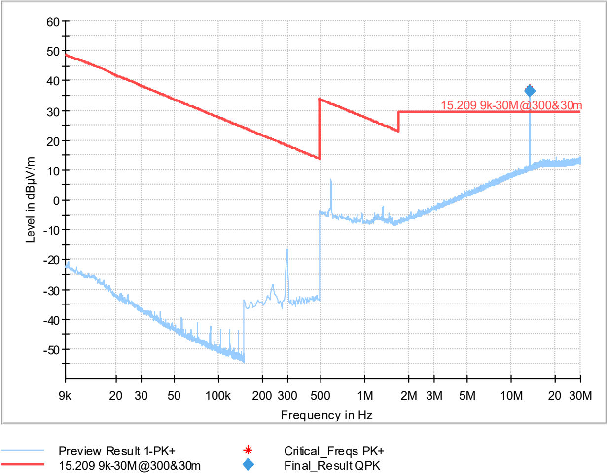
Plot no. 4: Radiated emissions 9 kHz – 30 MHz, EUT standing (see photos in annex B for EUT position)
