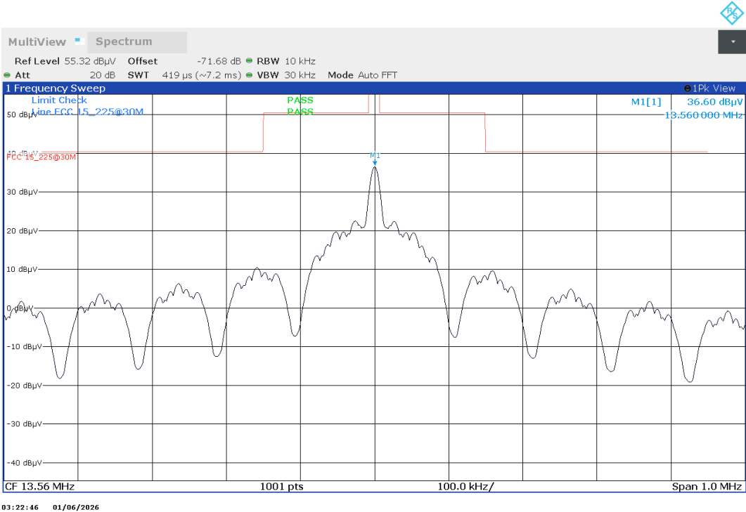
Plot no. 2: Transmitter Spectrum Mask (TSM), Set-up 2, Op. 2
