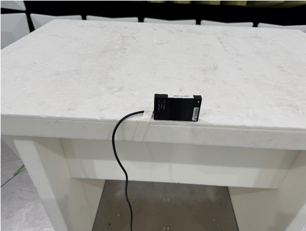
Photo No. 14, measurement in SAC, close view, EUT A + AE 1 standing:
