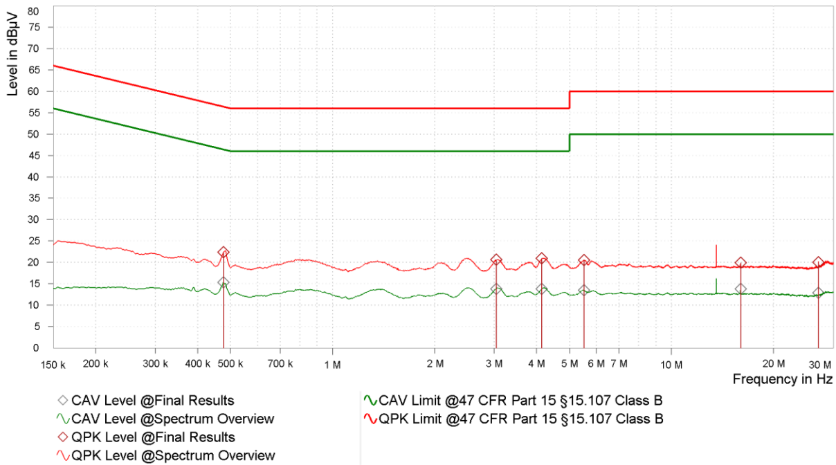
Plot No. 18: Conducted emissions, set-up 1, Op. 1, L1
