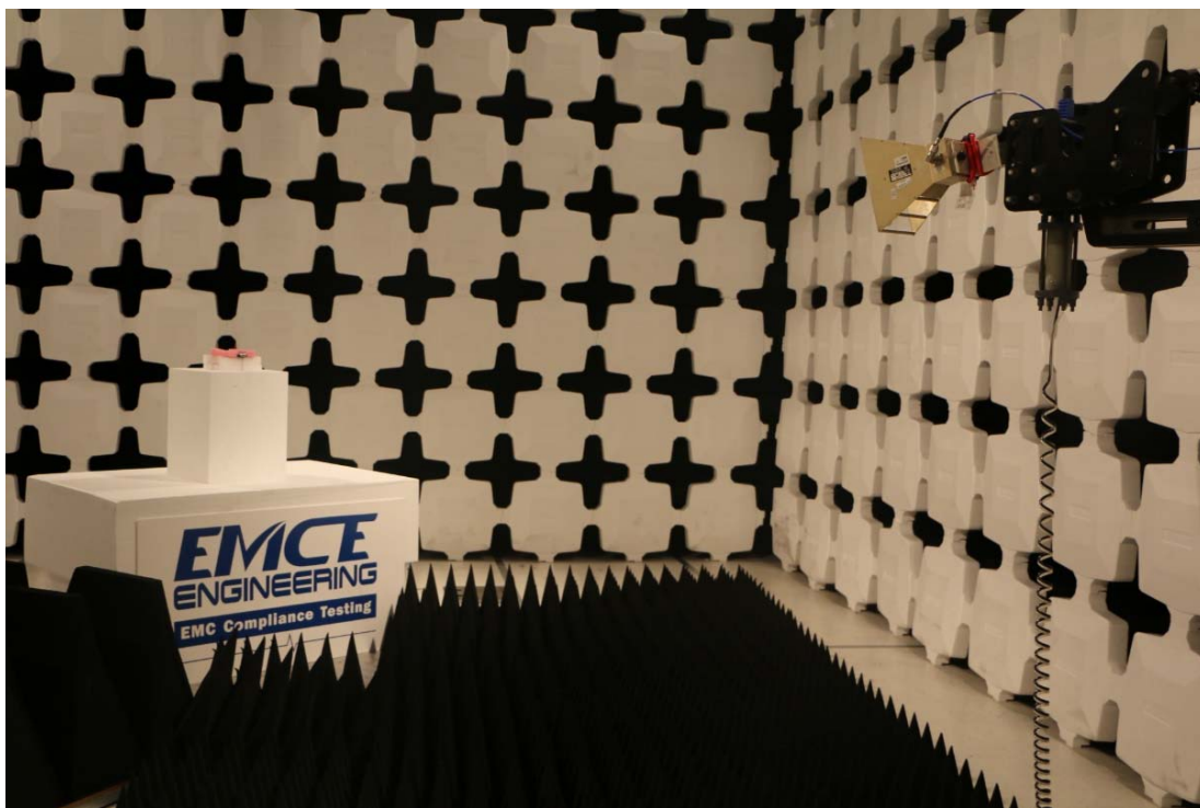
[Radiated Emissions 1 GHz – 25 GHz]
