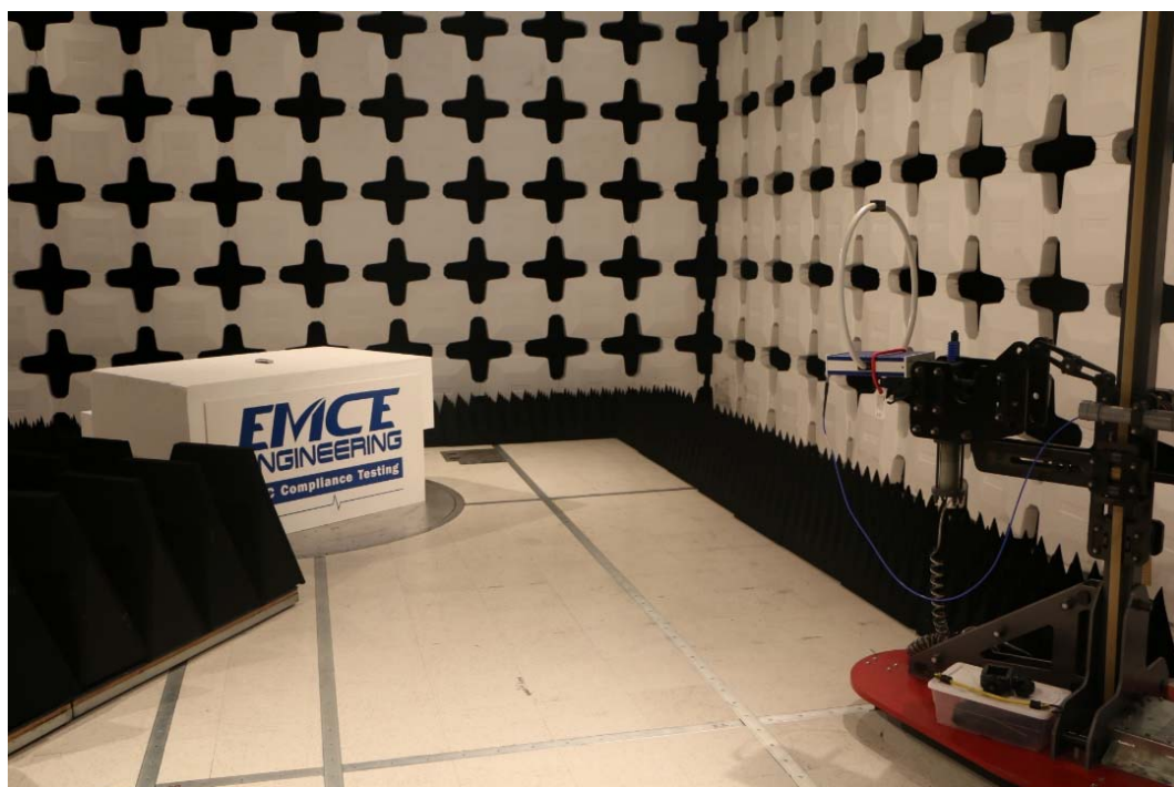
[Radiated Emissions 9 kHz – 30 MHz]
