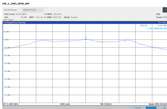
Figure 8.5-3: Conducted power spectral density reference level, 2402 MHz
