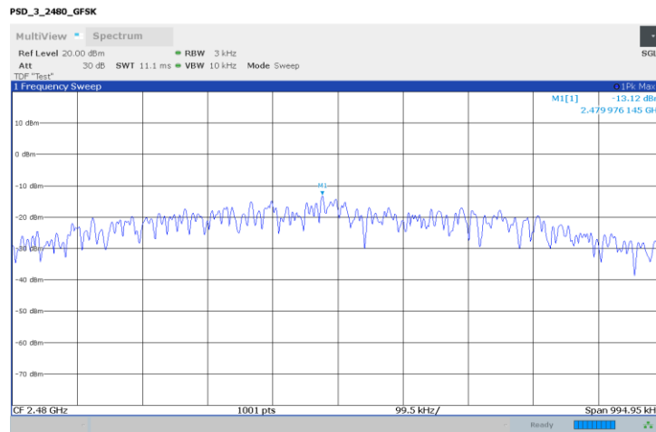
Figure 8.6-3: Power spectral density, 2480 MHz
