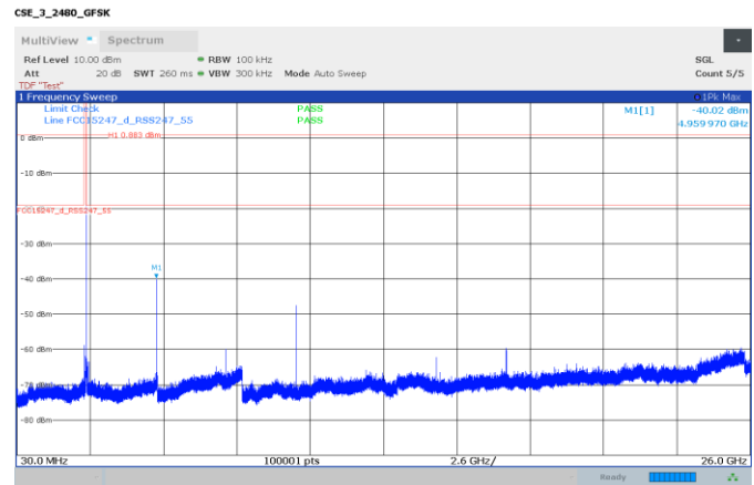
Figure 8.5-8: Antenna port conducted spurious emissions, 2480 MHz
