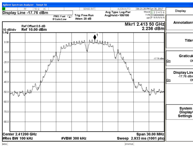
802.11b_Low Channel
