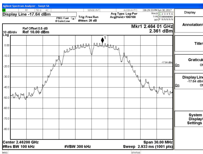
802.11b_High Channel
