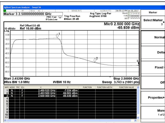
802.11g High channel(Average)
