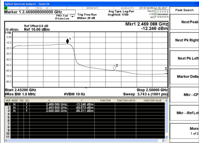
802.11n-HT40 High channel(Average)
