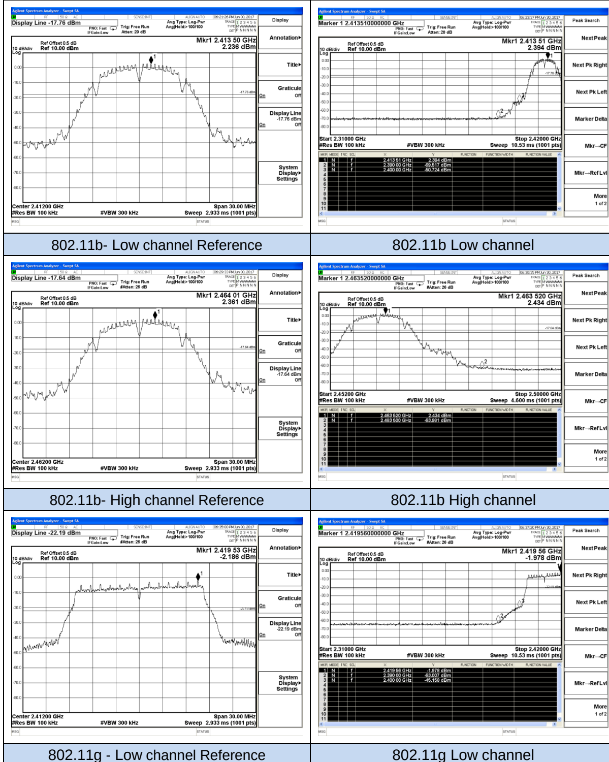
Test plot of Band Edges Test
