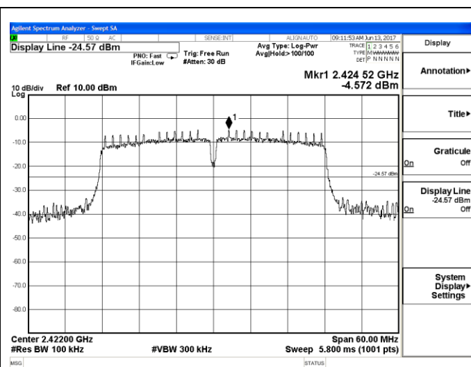
802.11n-HT40 Low channel
