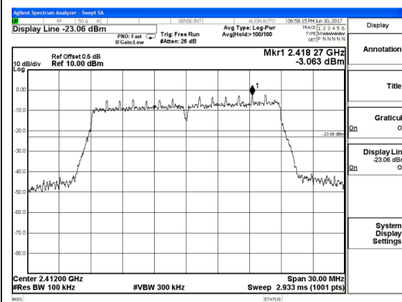
802.11n(HT20)- Low channel Reference
