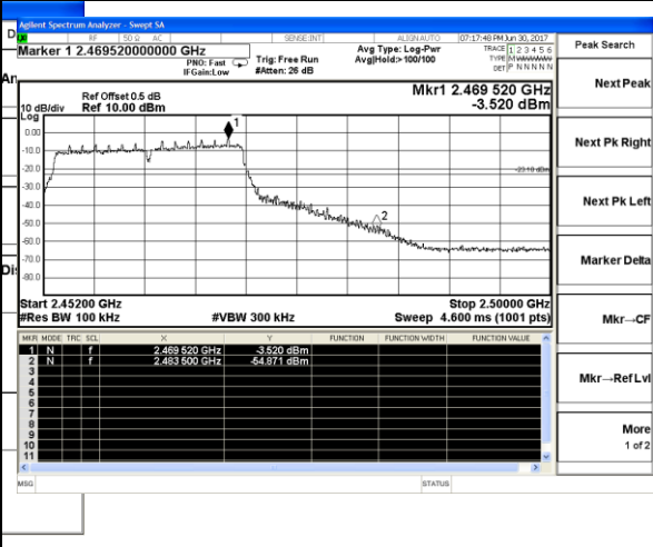
802.11n(HT20)-High channel
