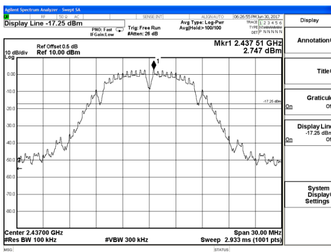
802.11b_Middle Channel
