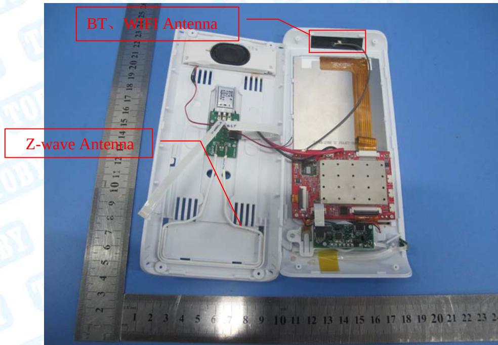
Photo 9 Internal of EUT
