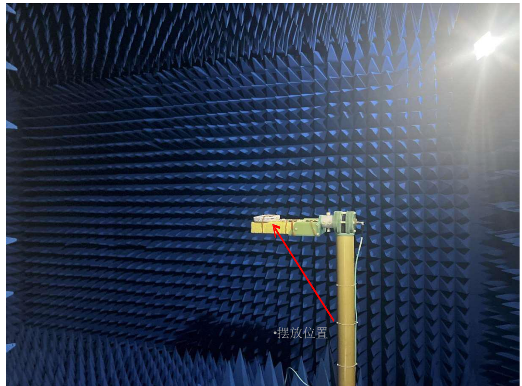
Product testing setup
