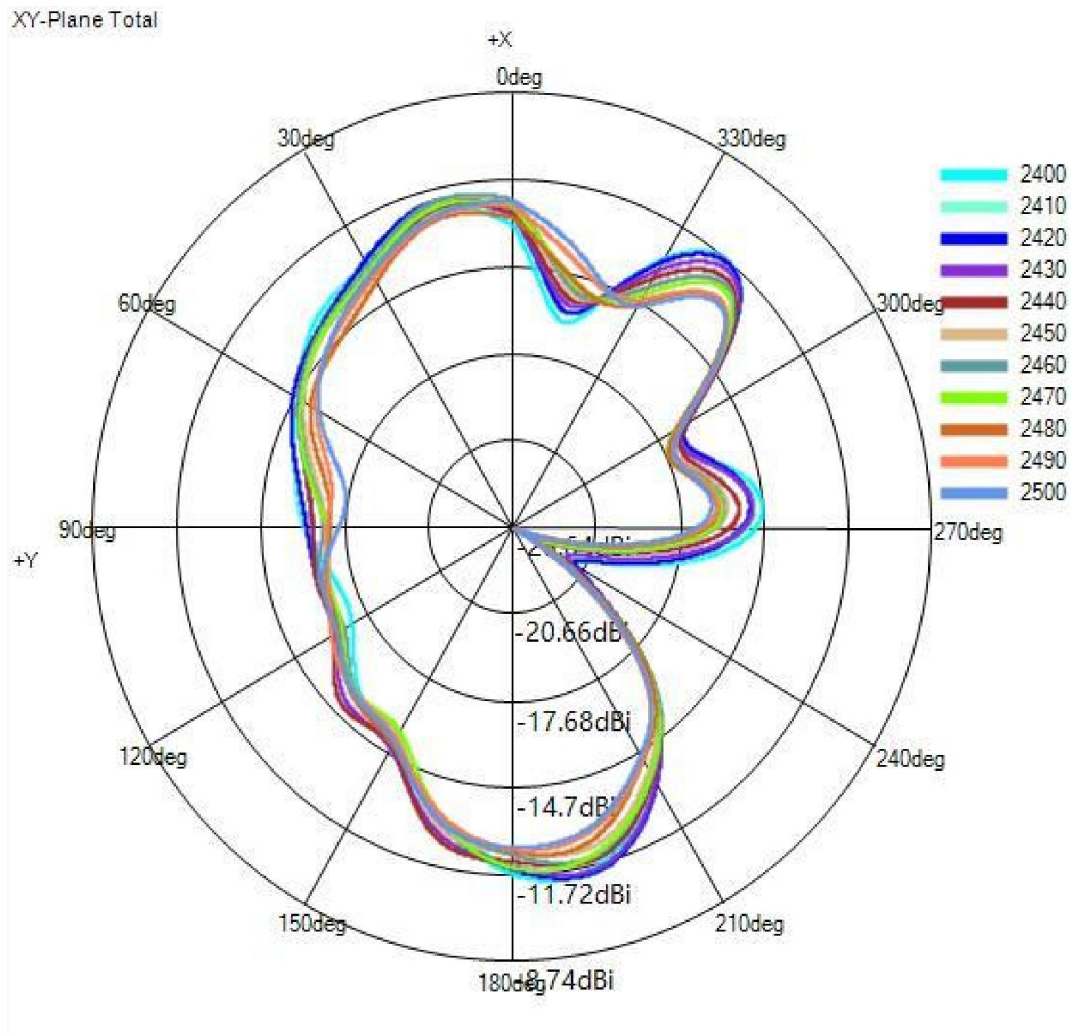
(3) X-Y Plane(unit:dBi):
