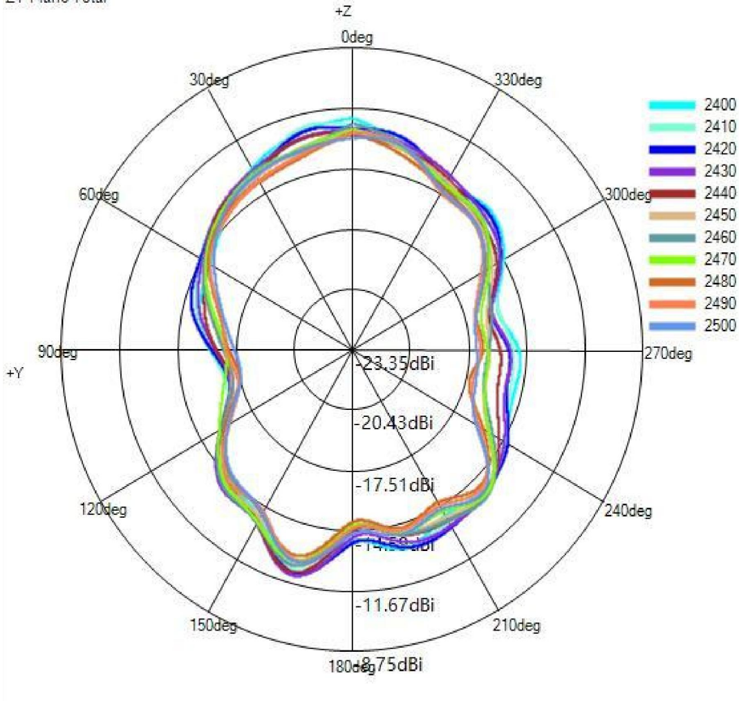
(2) Y-Z Plane(unit:dBi):
