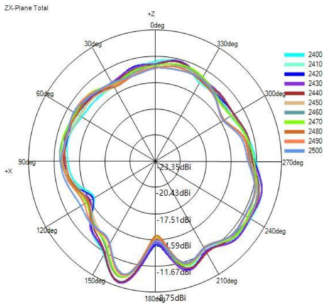
(1) X-Z Plane(unit:dBi):
