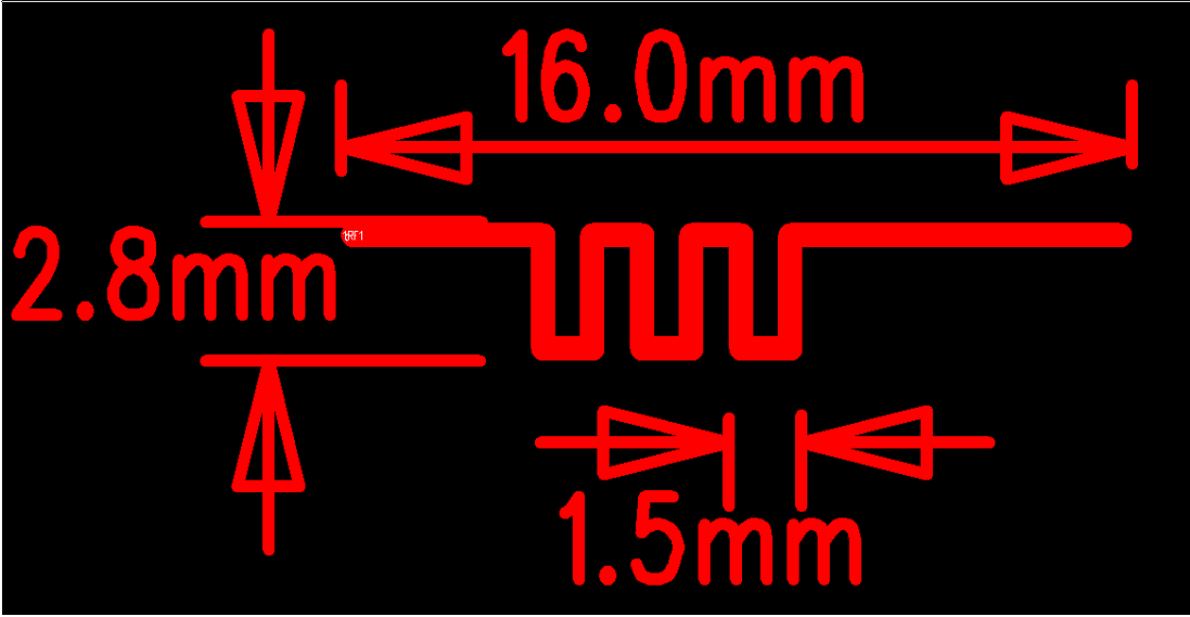
Antenna Photo & Length (mm)
