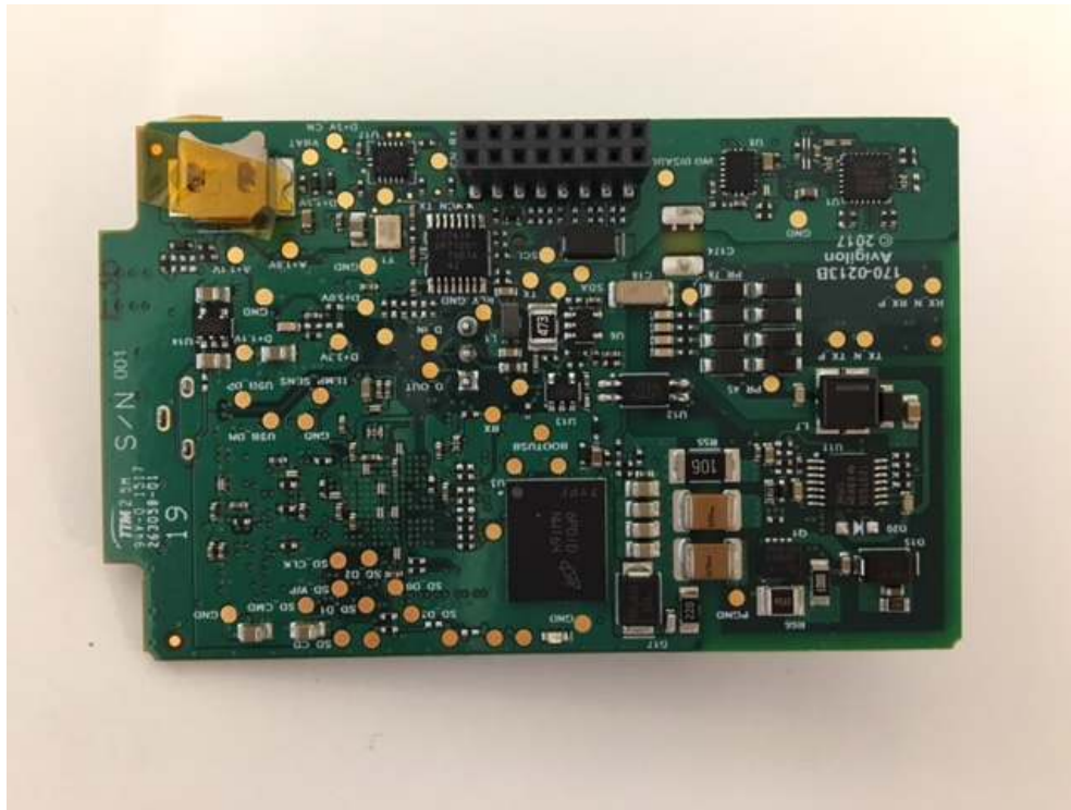
Avigilon Processor Board Bottom View:
