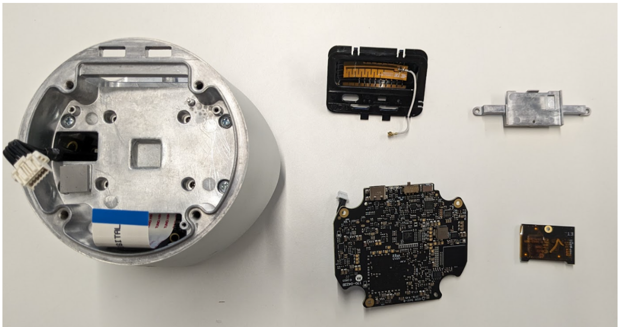
Internal Photo: Mainboard Bottom with Base Pan & IoT Hub Board Bottom & RF Antenna Shroud
