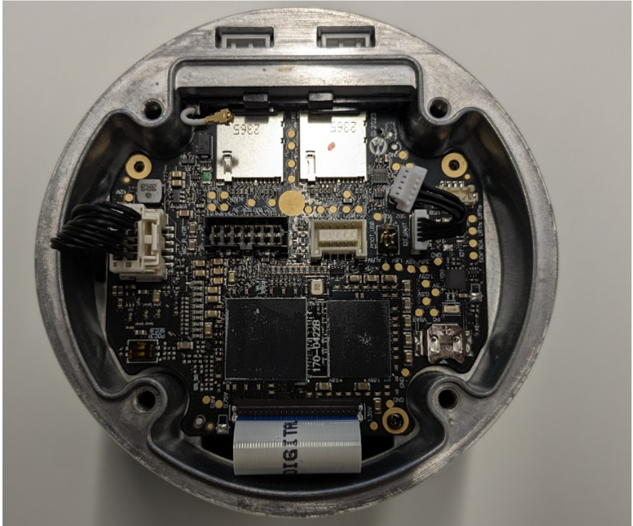
Internal Photo: Mainboard in Base Pan with IoT Hub Board Removed
