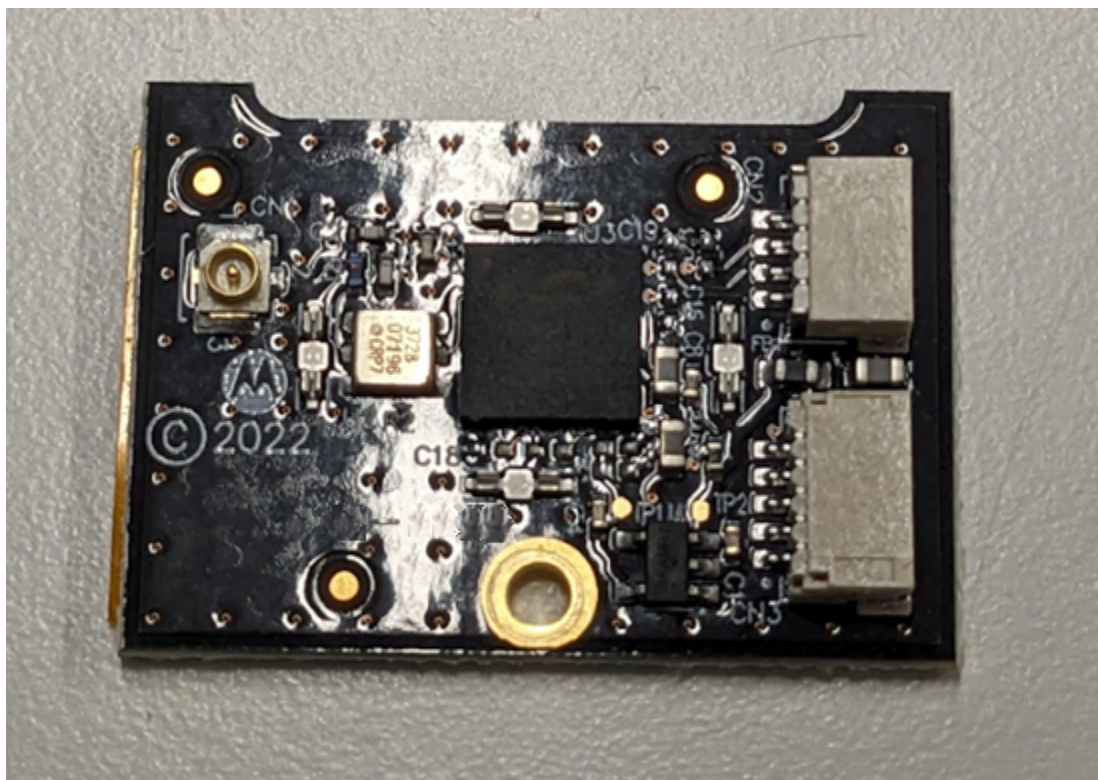
Internal Photo: Bottom of IoT Hub Board
