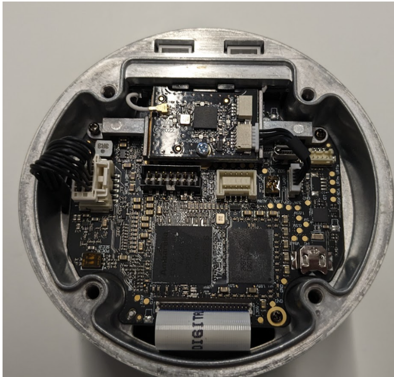
Internal Photo: Mainboard & IoT Hub Board in Shroud
