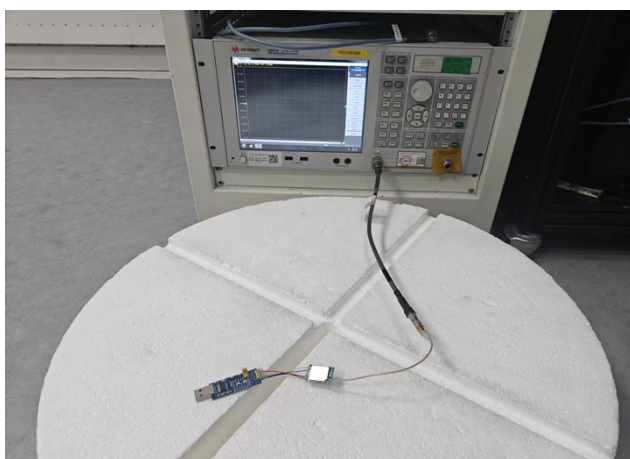
Free Space Impedance Setup
