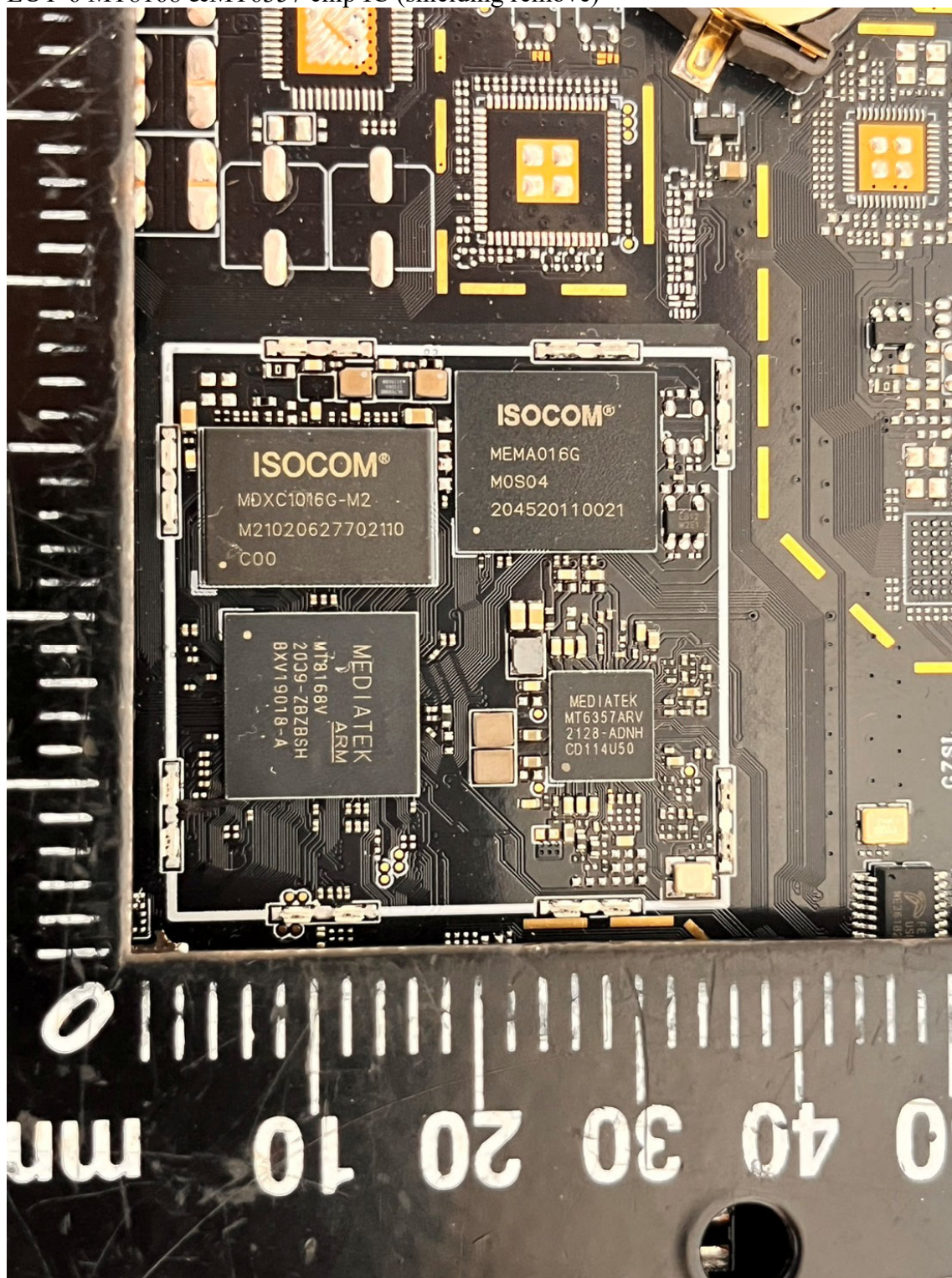
EUT-6 MT8168 & MT6357 chip IC (shielding remove)
