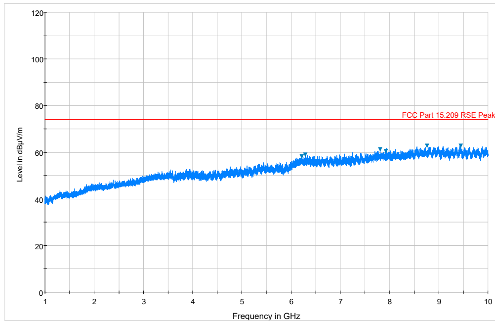
Plot 7-44. Radiated Spurious Plot above 1GHz (125kHz, Low Channel, Ant. Pol. H)
