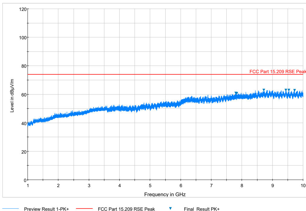
Plot 7-38. Radiated Spurious Plot above 1GHz (500kHz, Low Channel, Ant. Pol. H)
