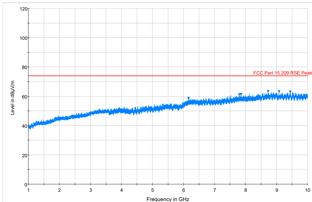
Plot 7-45. Radiated Spurious Plot above 1GHz (125kHz, Low Channel, Ant. Pol. V)
