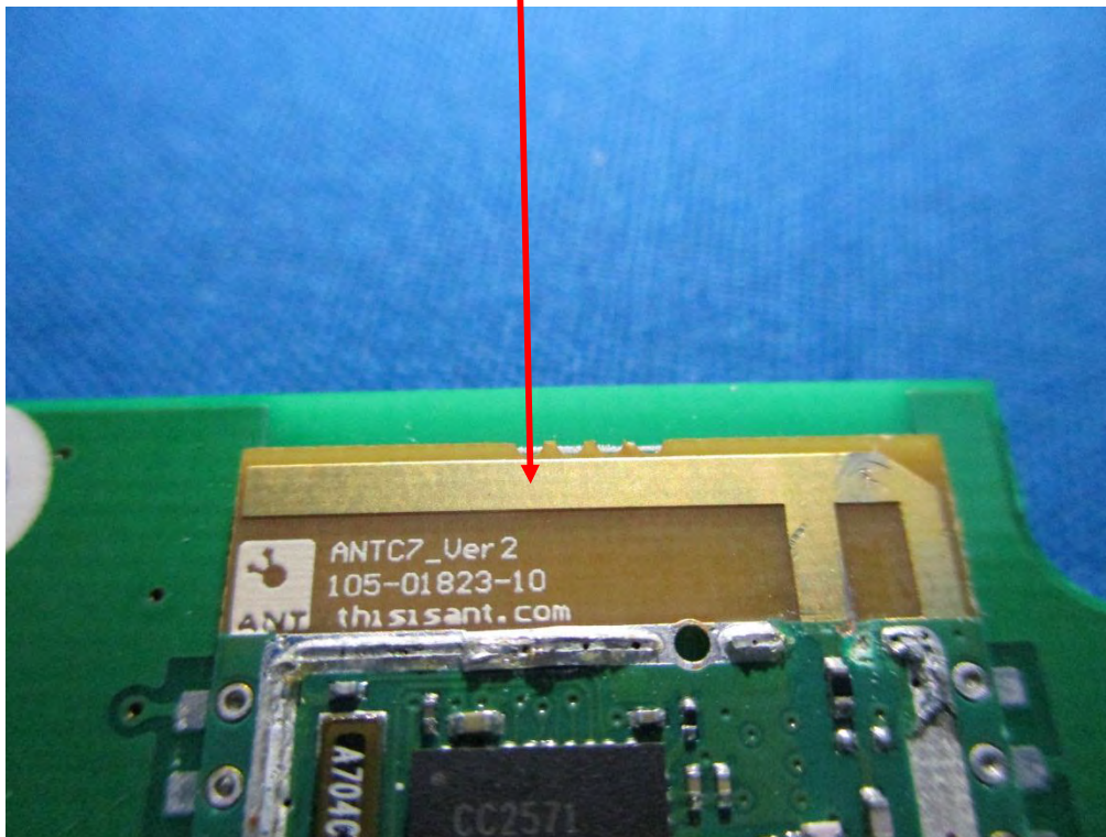
ANT+ Antenna – Top View
