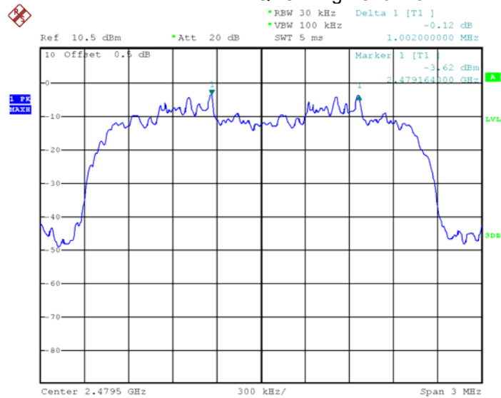
Pi/4 DQPSK High Channel
