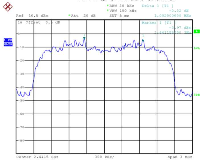
Pi/4 DQPSK Middle Channel
