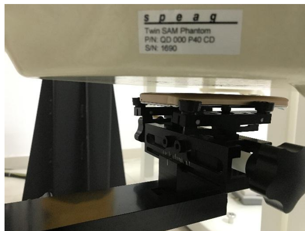
Hotspot mode - Rear Side (10mm)
