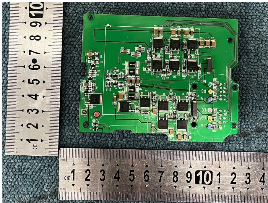
SECONDARY BOARD 1 REAR VIEW (WITHOUT SHIELDING)
