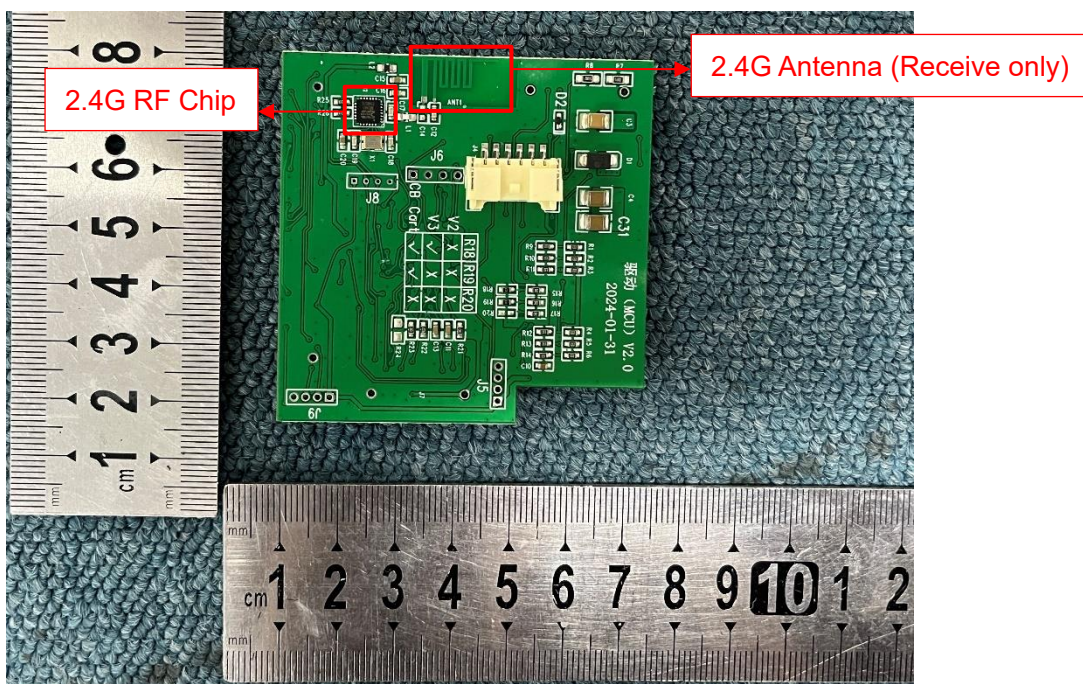
SECONDARY BOARD 5 TOP VIEW
