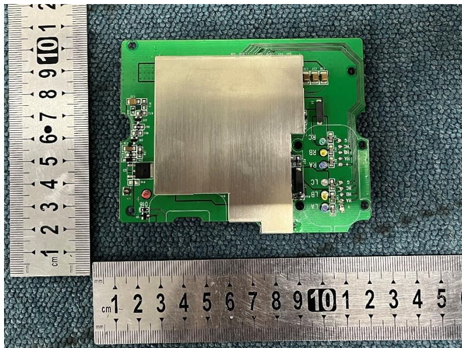
SECONDARY BOARD 1 REAR VIEW (WITH SHIELDING)
