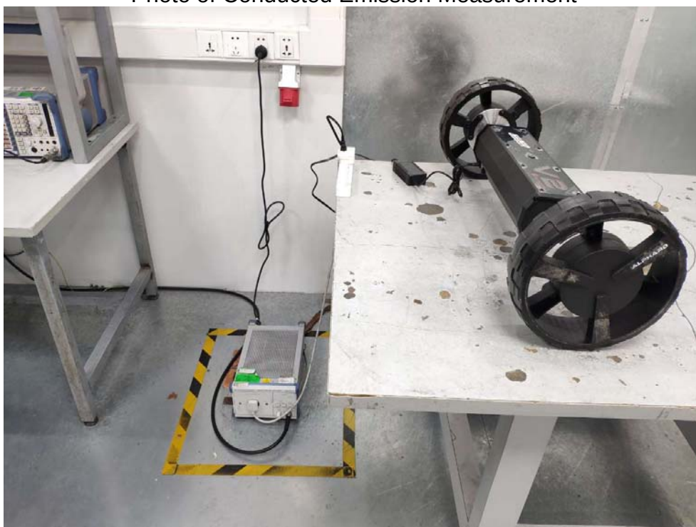
FCC ID: 2ANDF-V2 Photo of Conducted Emission Measurement
