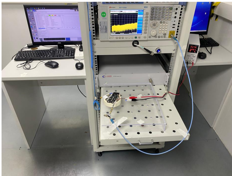
Conducted Test-2.4G
