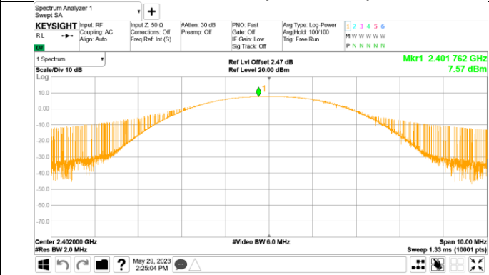
Channel 0 (2402MHz)
