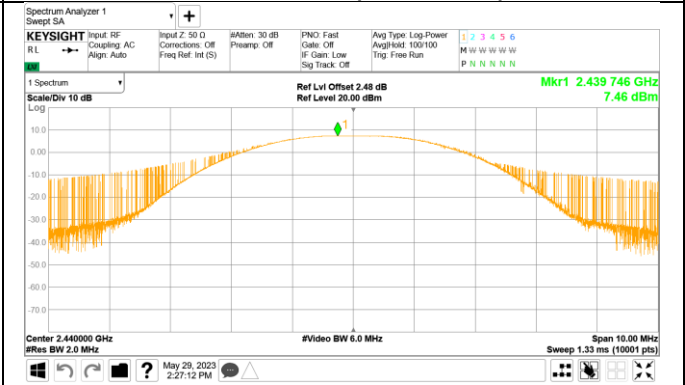
Channel 19 (2440MHz)
