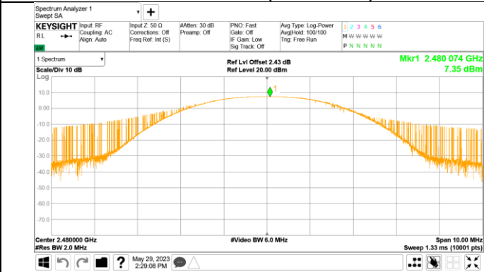
Channel 39 (2480MHz)
