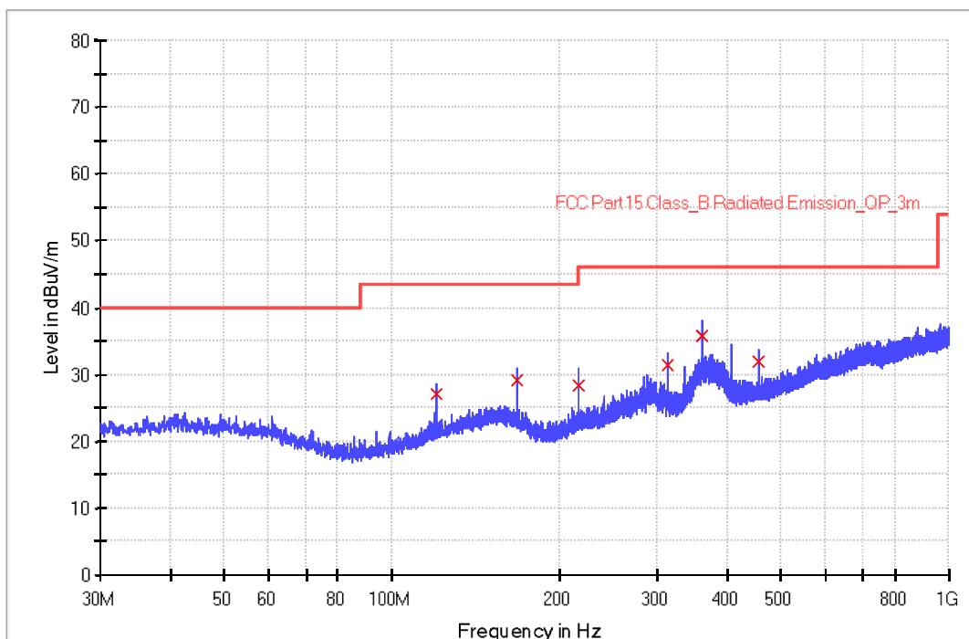
RE_VULB9168_pre_Cont_30-1000
