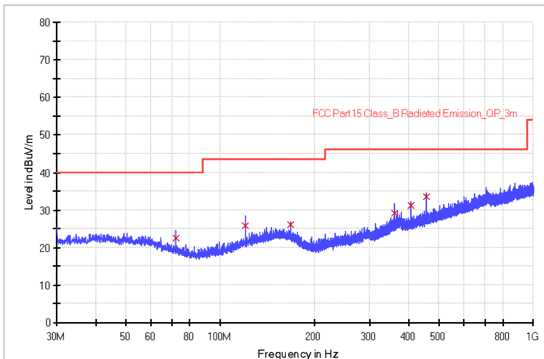
PE_VULB9168_pre_Cont_30-1000
