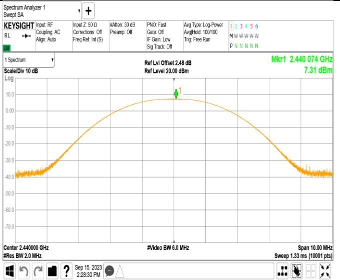
Channel 19 (2440MHz)
