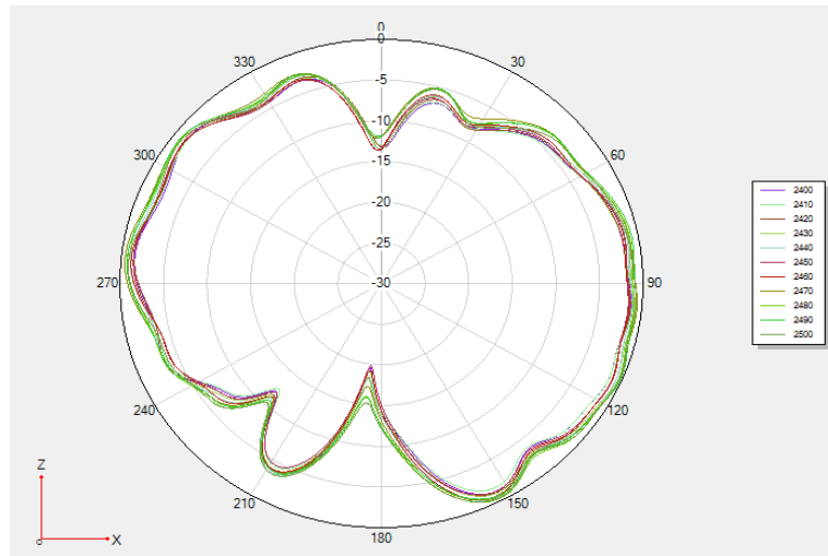
Phi 90 2D
