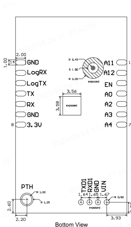
Bottom View
