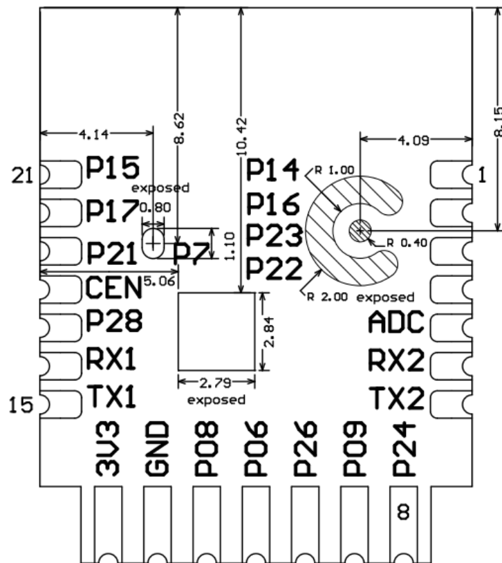
Bottom View
