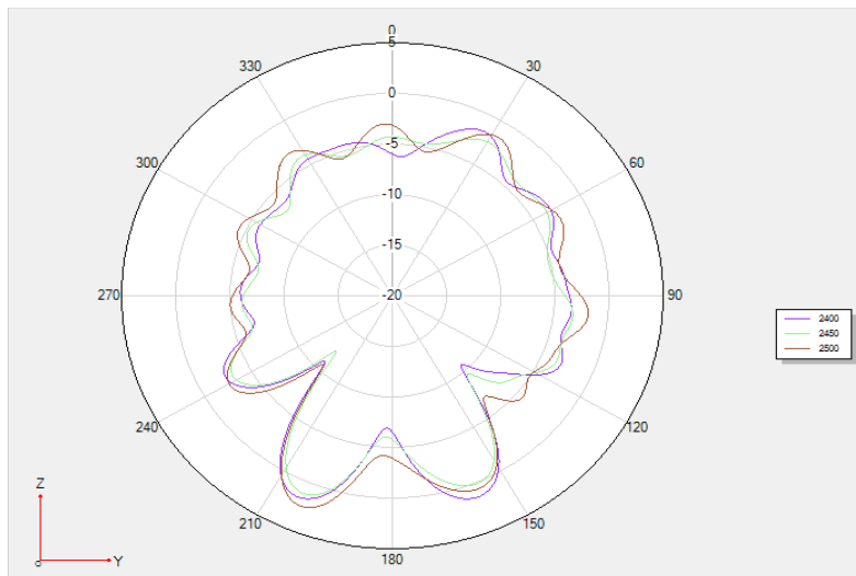
Theta 90 2D
