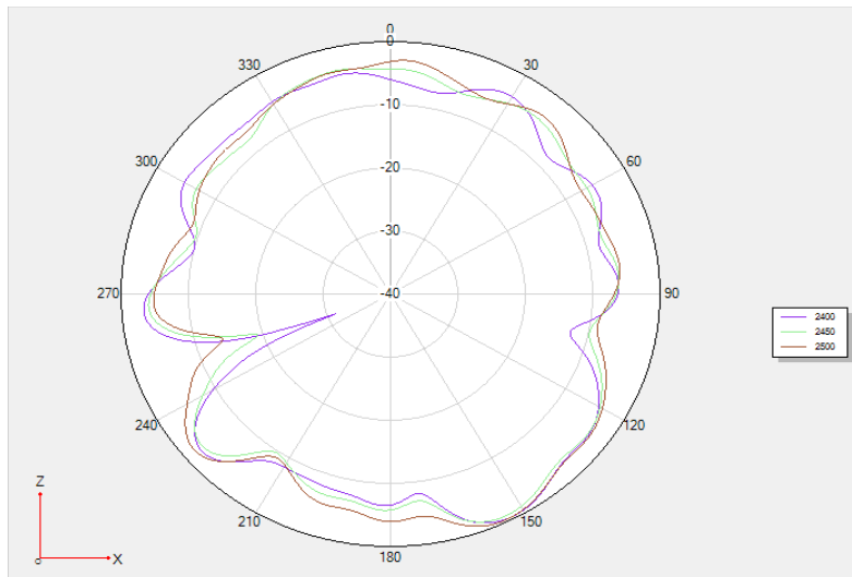
Phi 90 2D
