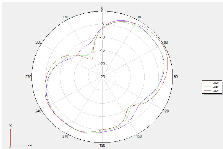
Theta 90 2D
