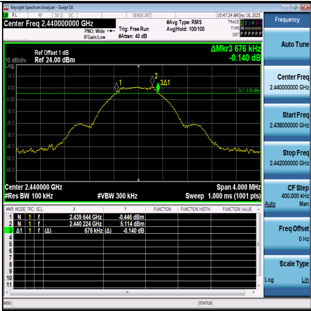
BLE_1M-Ant1-2440-PASS
