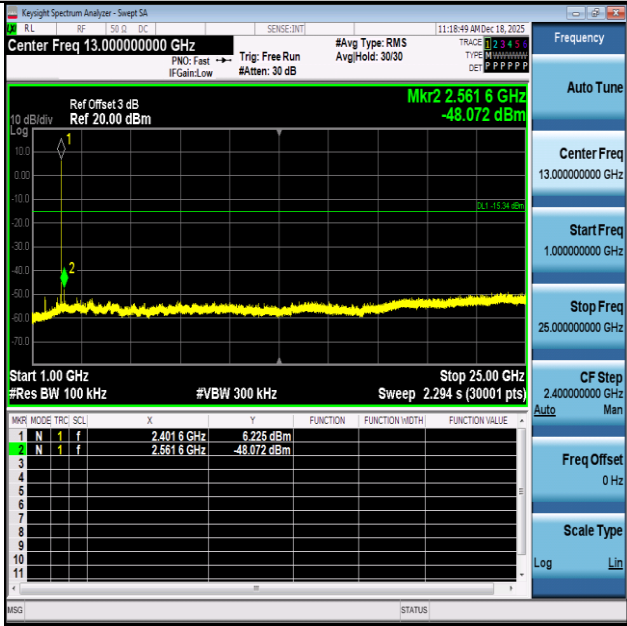
BLE_125K-Ant1-2402-1000~25000-PASS
