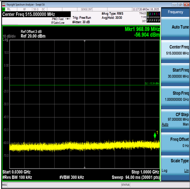
BLE_125K-Ant1-2402-30~1000-PASS
