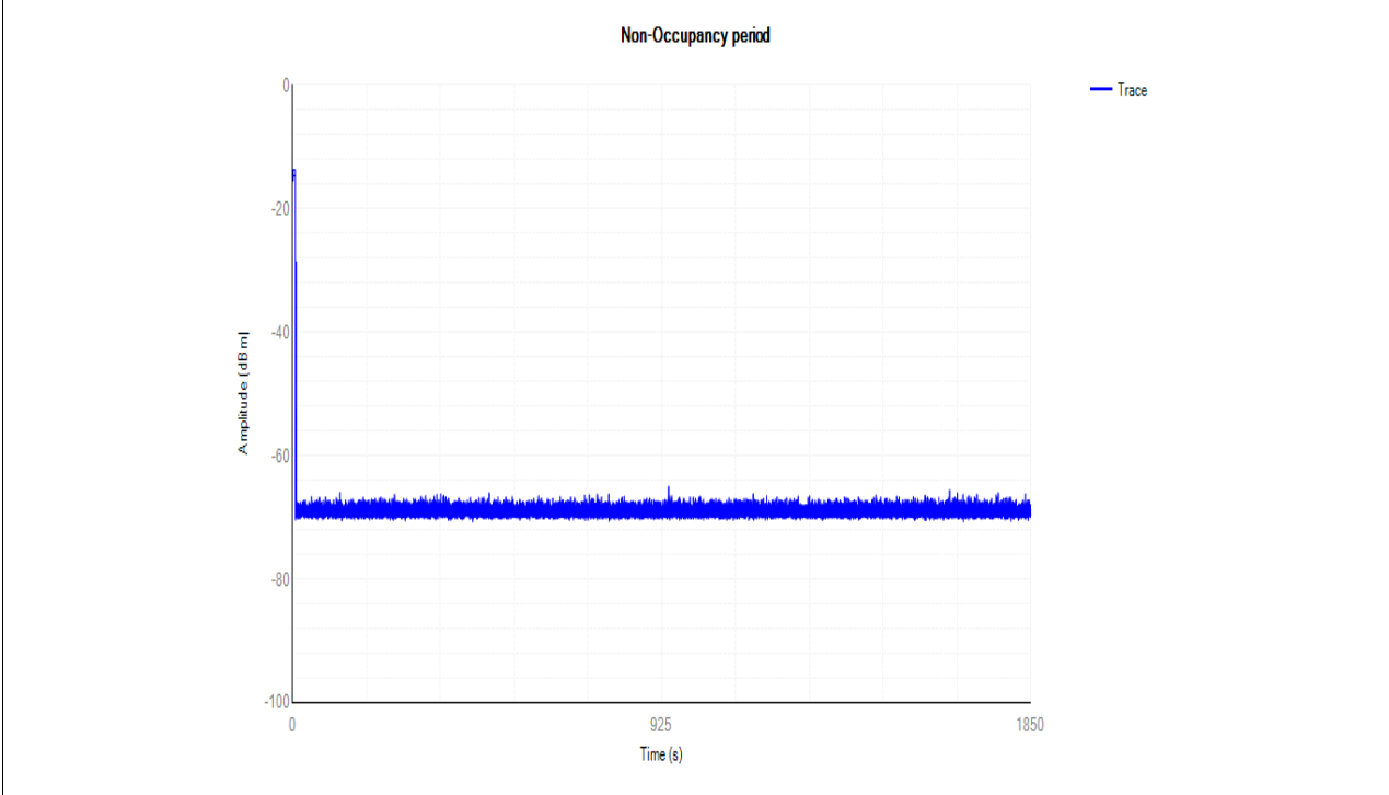
n20 5500MHz Non-Occupancy
