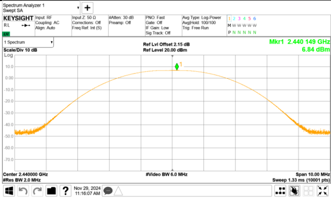
Channel 19 (2440MHz)
