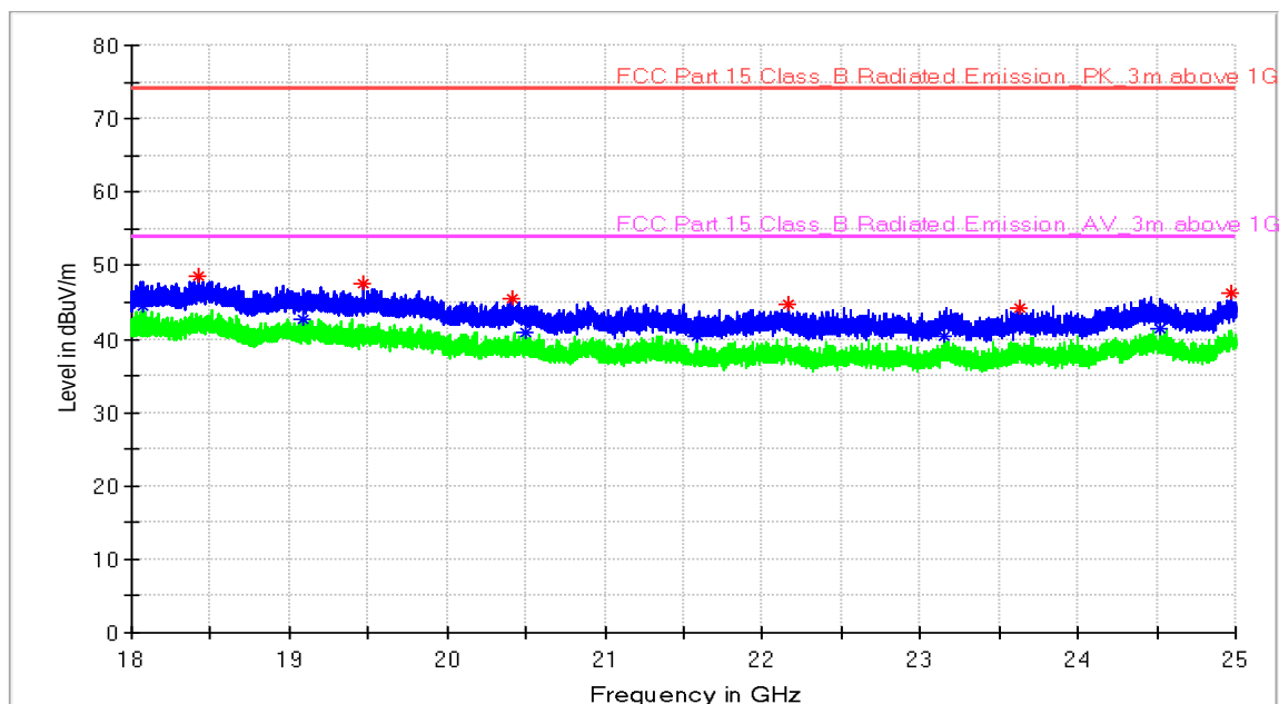
Full Spectrum
