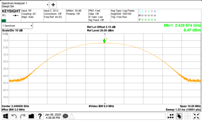
Channel 19 (2440MHz)
