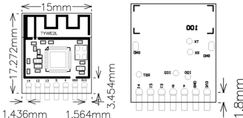
Figure 3 TYWE2L front view and rear view
