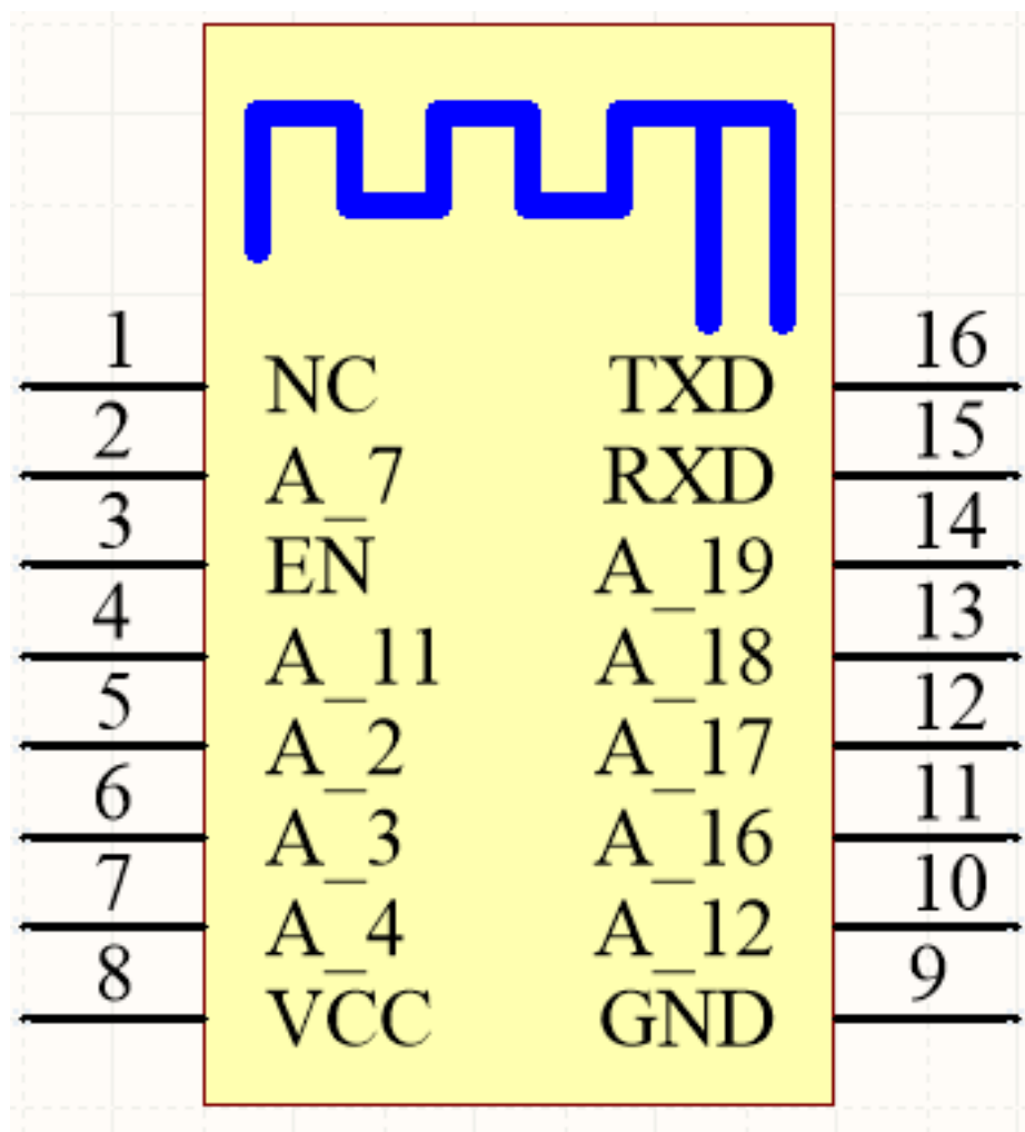
WBR3-PRO PCB footprint
