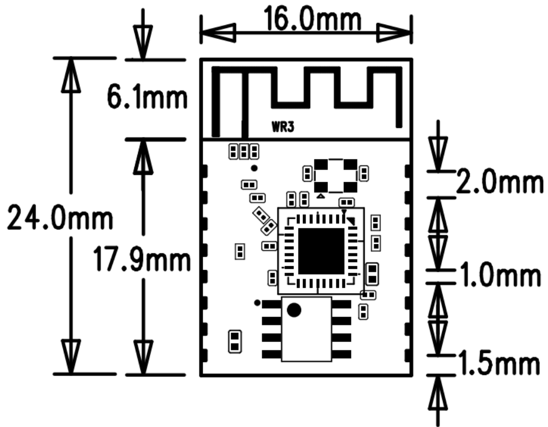
Figure 6.1. Top view of the module
