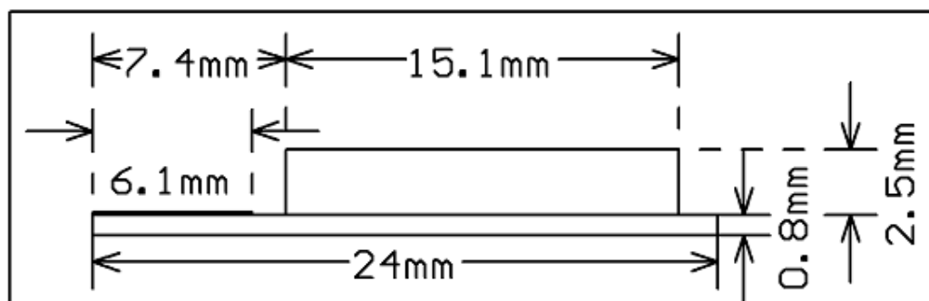
Figure 6.2. The module's mechanical view
