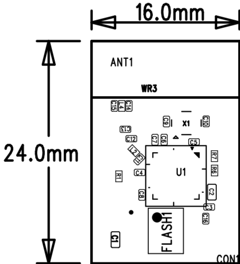
Figure 2.1. The dimensions of WR3
