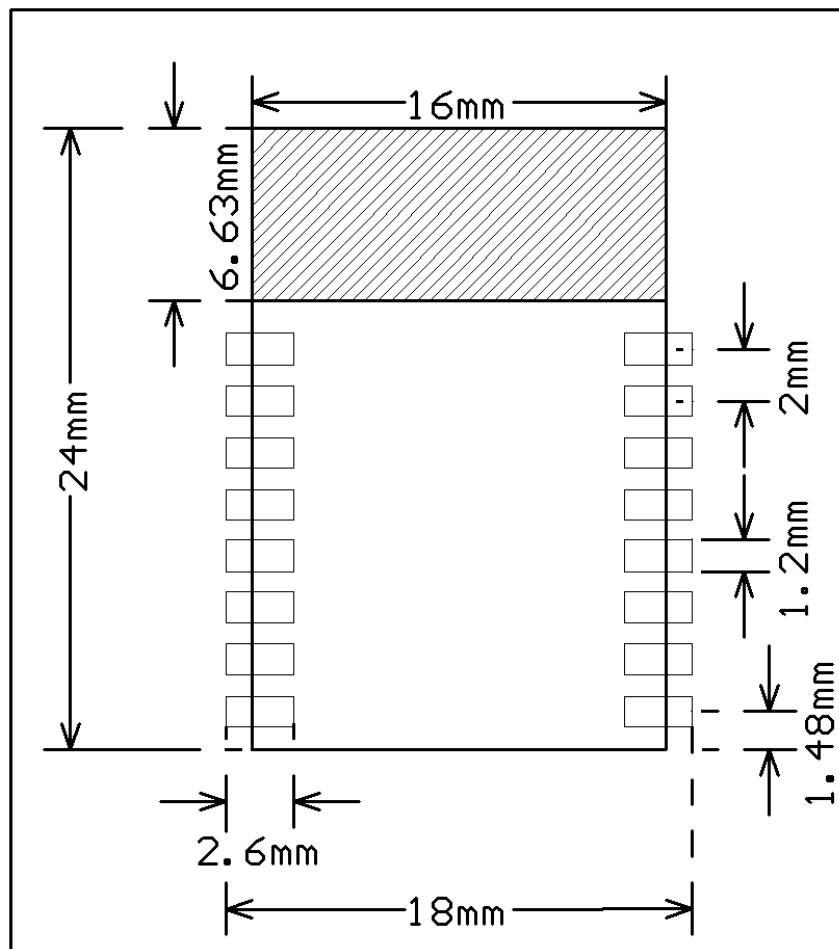
Figure 6.3. PCB footprint
