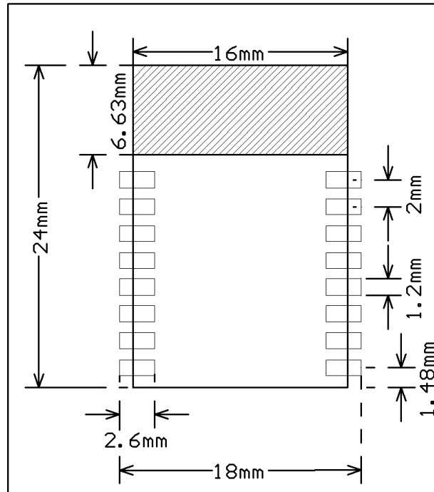
Figure 6-4 Layout of the PCB to which WRD3L applies
