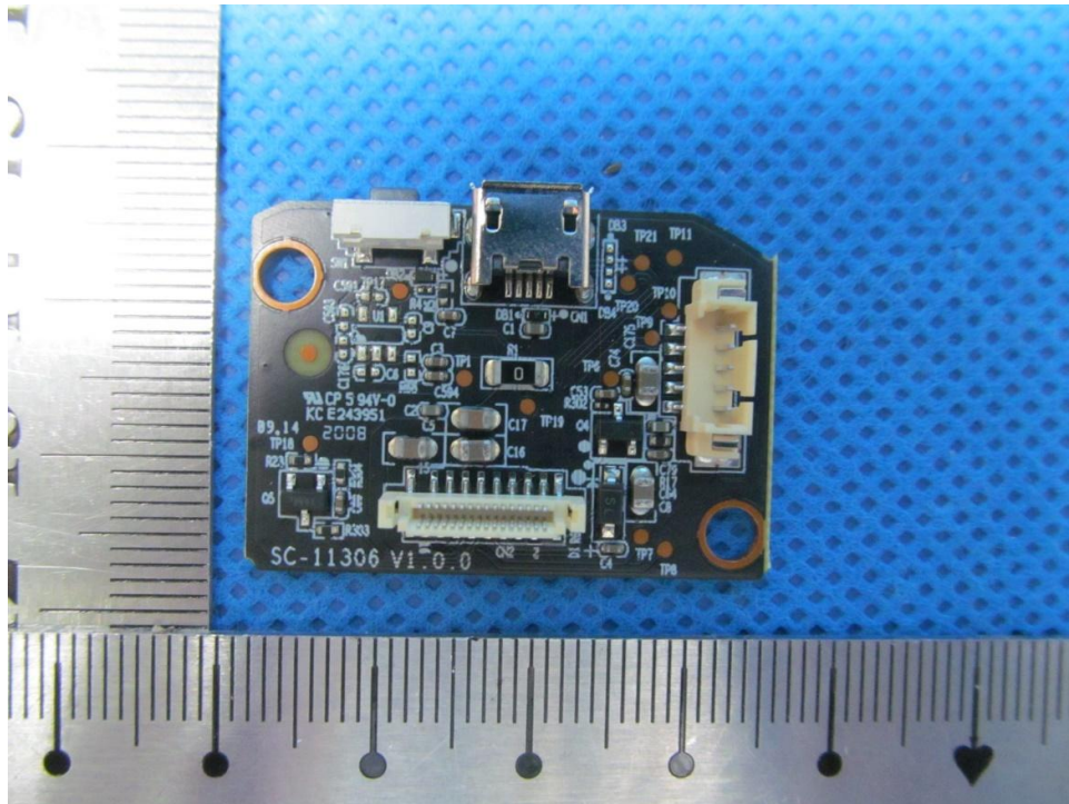
Photo 12. PCB view
