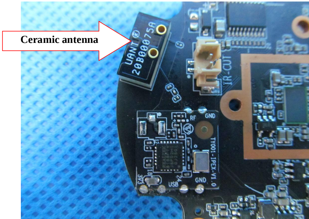
Photo 2. PCB view
