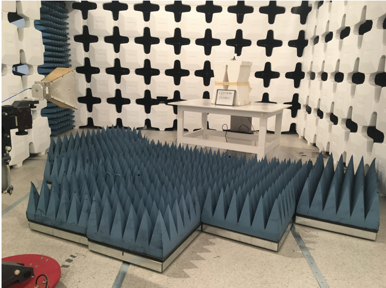
Figure 5. External Antenna Radiated Emissions, Above 1 GHz
