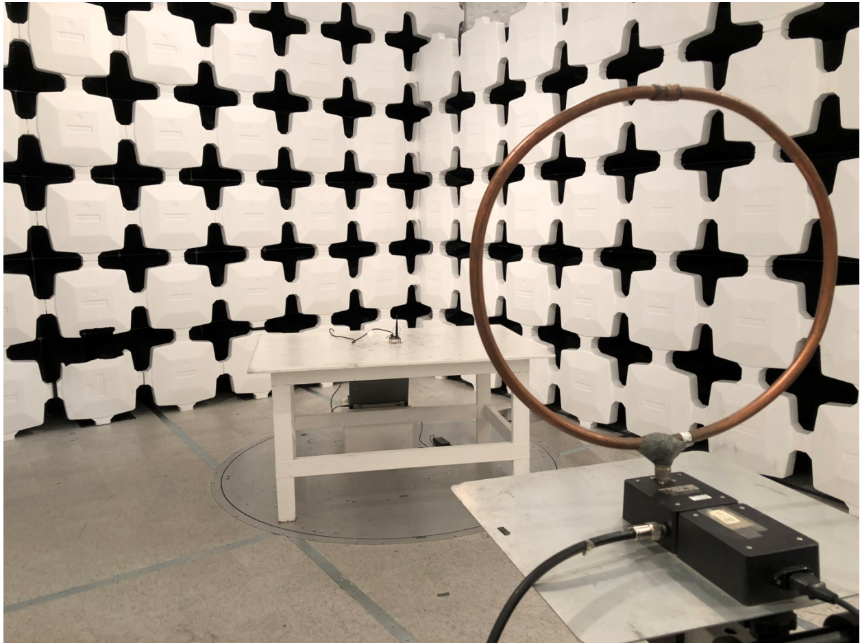
Figure 2. Spurious Radiated Emissions Below 30 MHz
