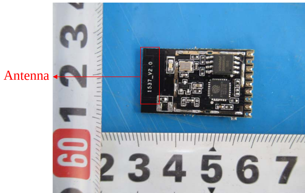
EUT – Wi-Fi Module Bottom View
