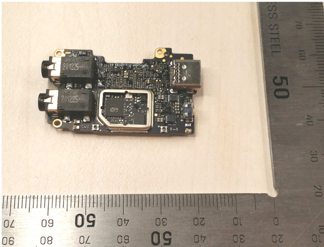
Figure 4: Mainboard view -1
