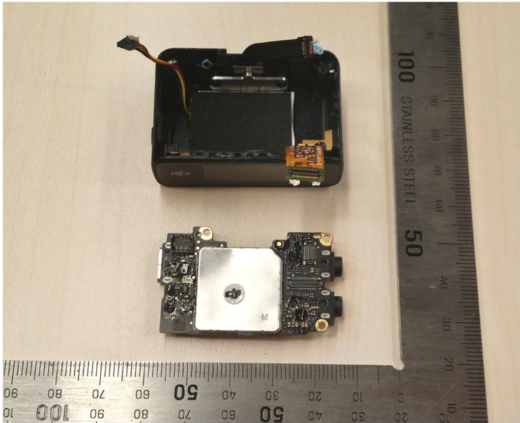
Figure 3: Internal view -3
