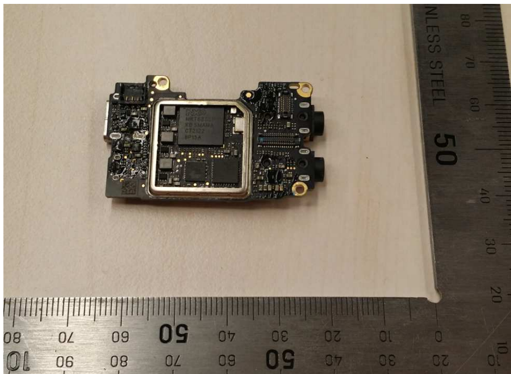
Figure 5: Mainboard view -2
