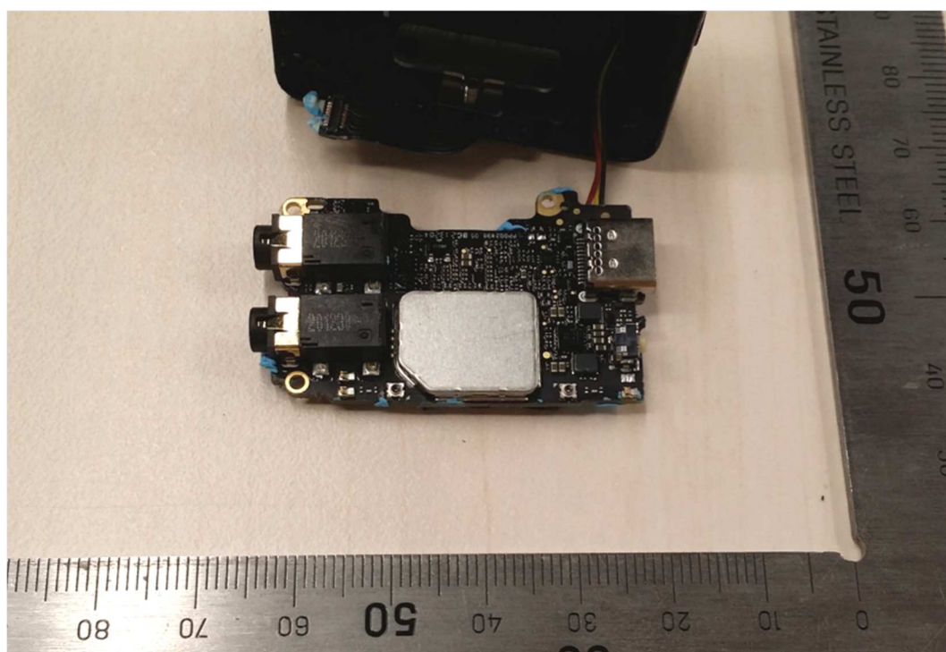
Figure 2: Internal view -2
