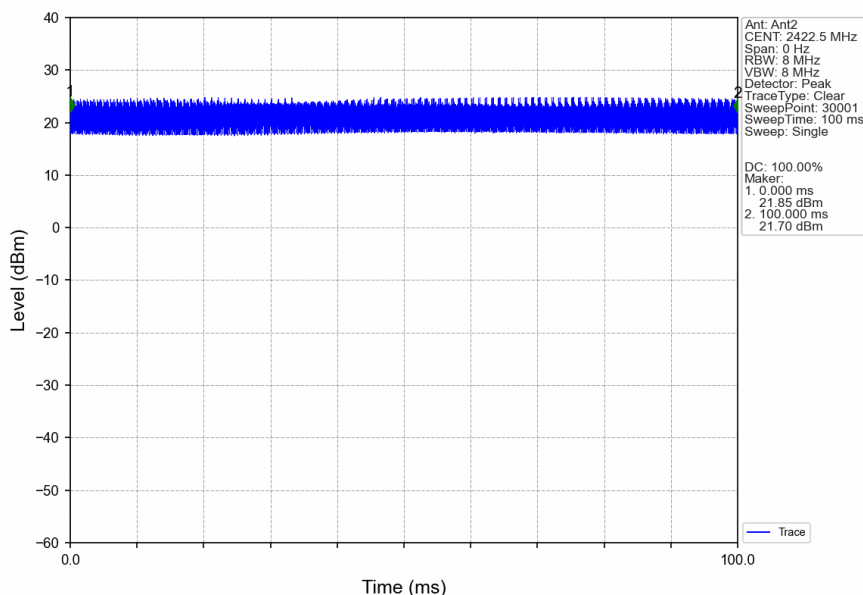
40M_LCH_2422.5MHz_Ant2_NTNV
