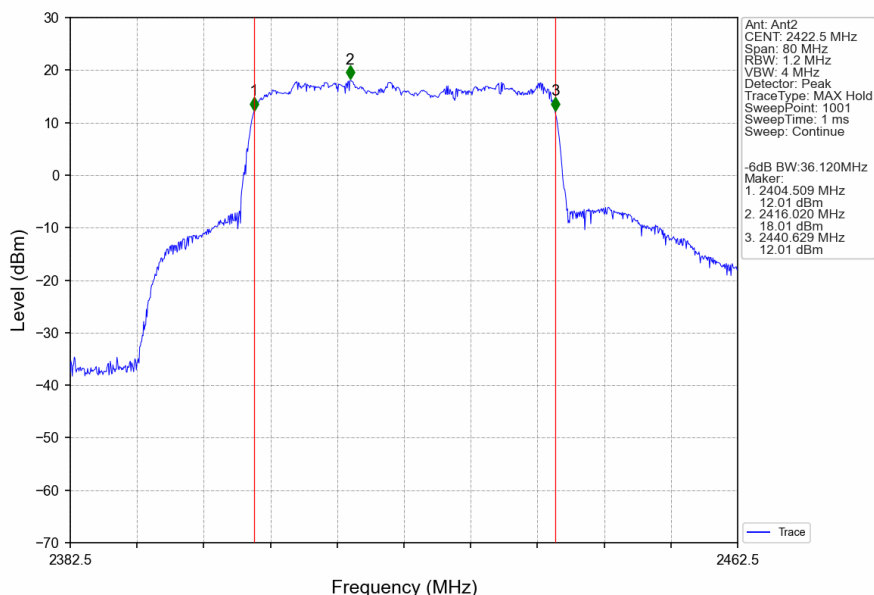
40M_LCH_2422.5MHz_Ant2_NTNV
