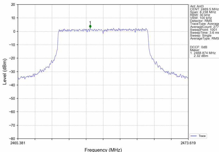
5M_HCH_2469.5MHz_Ant3_NTNV
