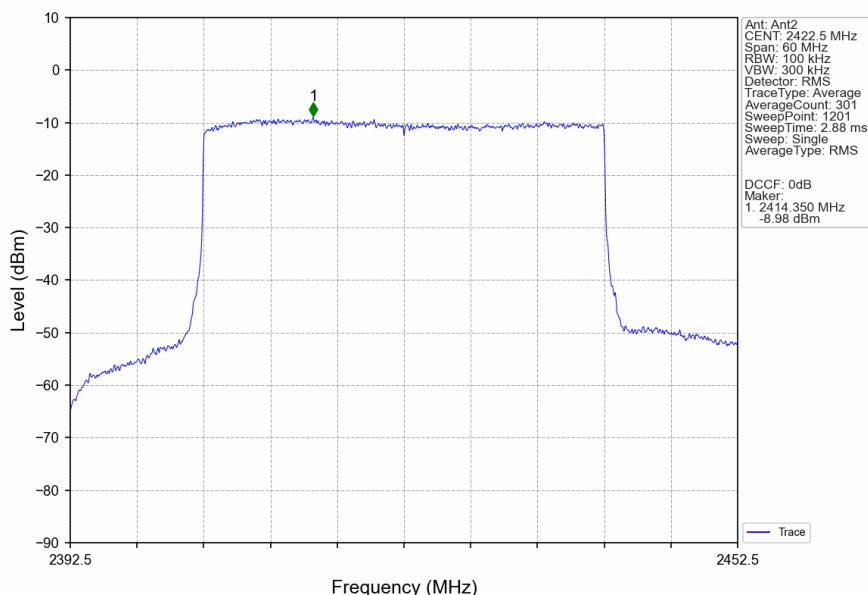
40M_LCH_2422.5MHz_Ant2_NTNV
