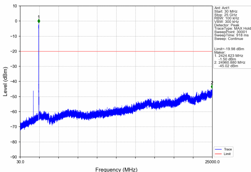
40M_LCH_2422.5MHz_Ant1_NTNV
