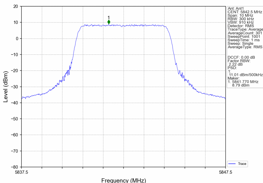
5G 5M B3_HCH_5842.5MHz_Ant1_NTNV
