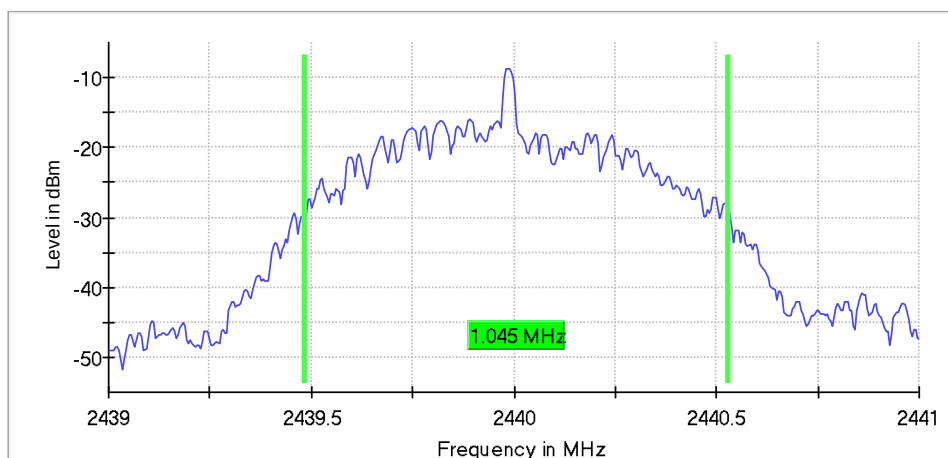
99 % Bandwidth
