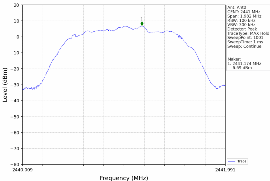
8DPSK_3DH5_MCH_2441MHz_Ant0_NTNV
